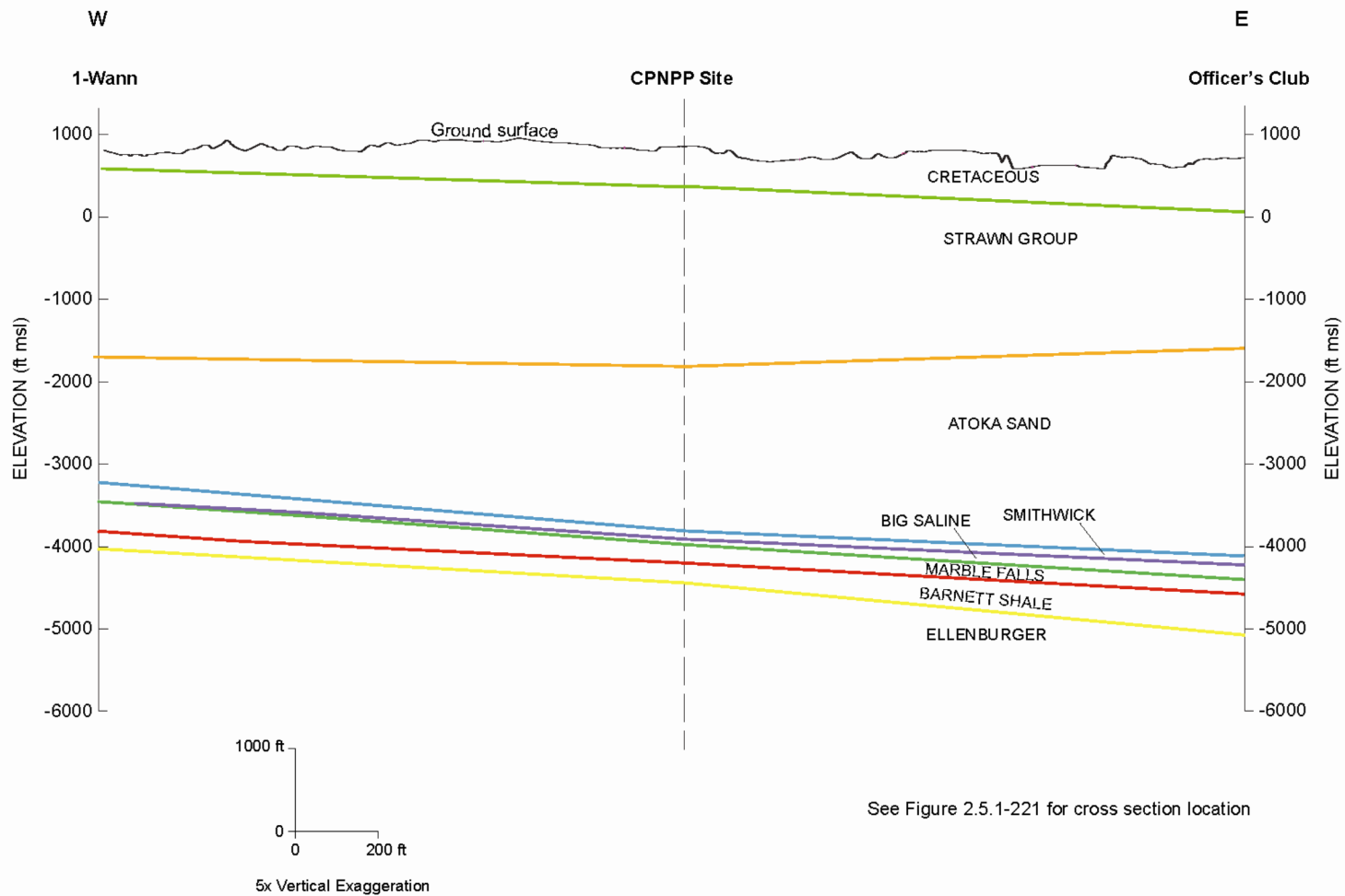
Figure 2.5.1-222 West-East Cross Section
