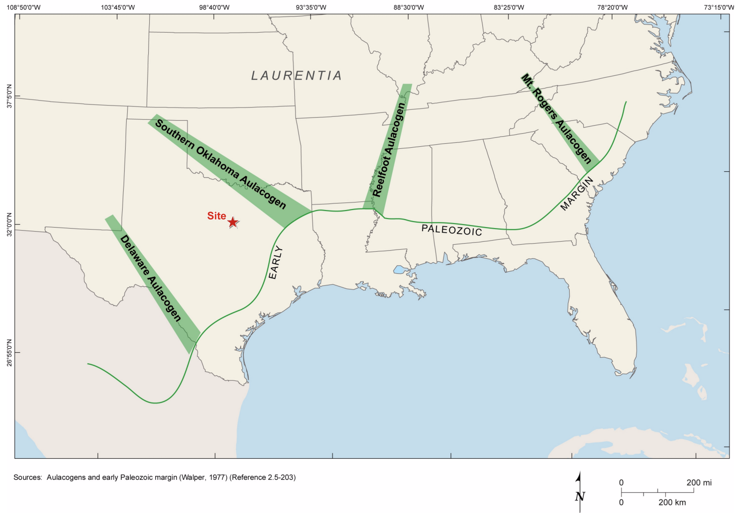
Figure 2.5.1-208 North American Aulacogens
