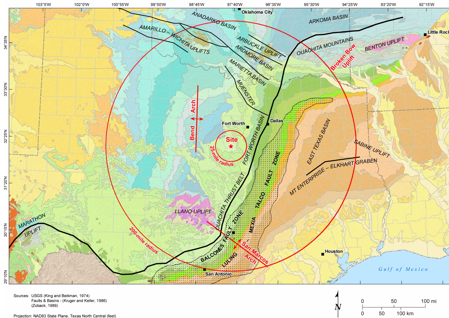
Figure 2.5.1-207 Regional Tectonic Features
