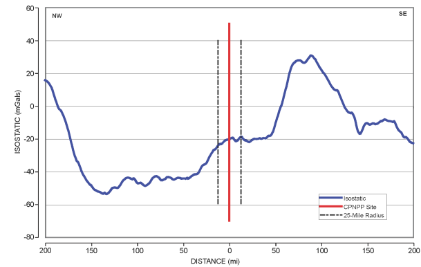
Figure D – Isostatic Gravity Profile
