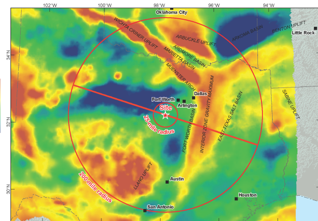
Figure C – Isostatic Gravity Map
