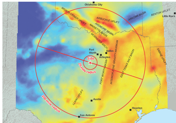
Figure A – Bouguer Gravity Map
