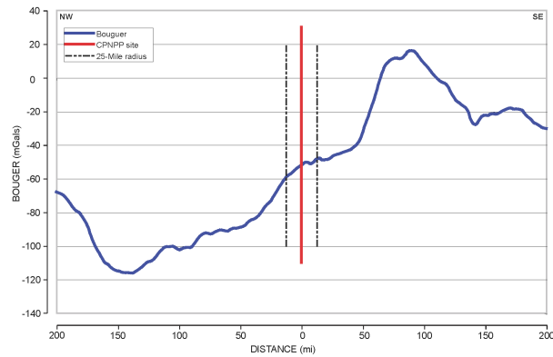
Figure B – Bouguer Gravity Profile
