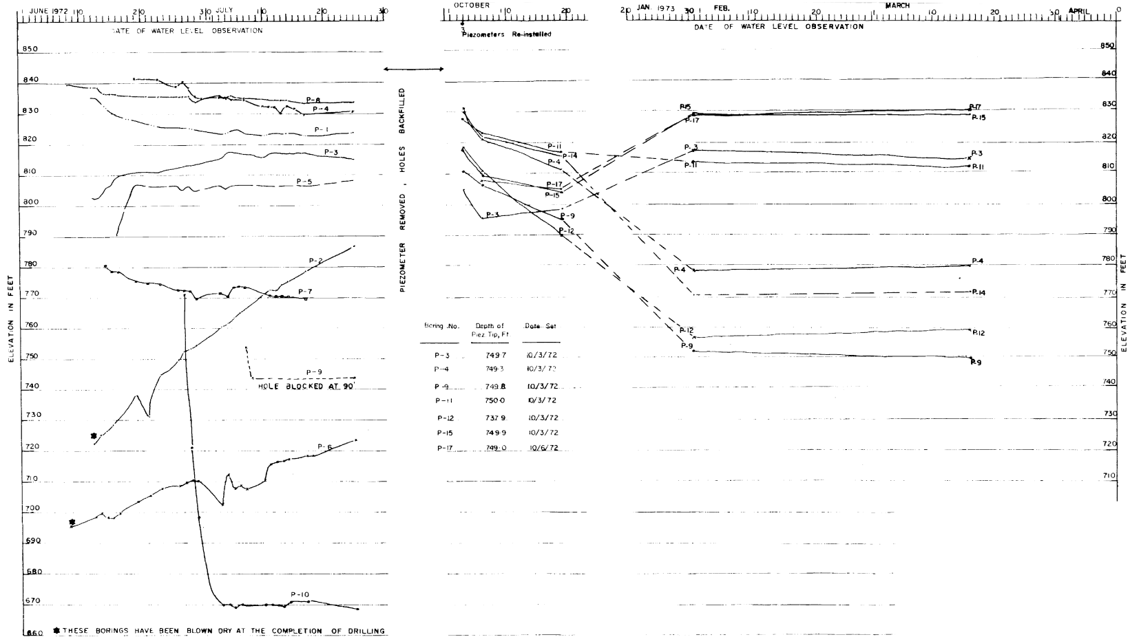
Figure 2.4.12-207 Historical Water Level Elevations
