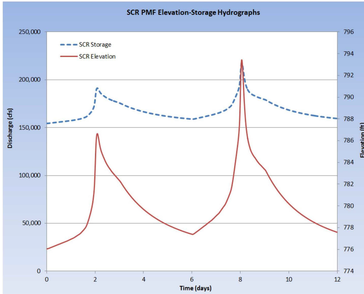
Figure 2.4.3-208 SCR Probable Maximum Flood Elevation Storage Hydrograph
