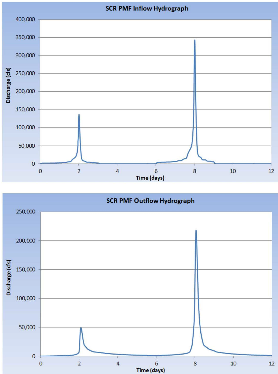
Figure 2.4.3-207 SCR Probable Maximum Flood Inflow Outflow Hydrographs
