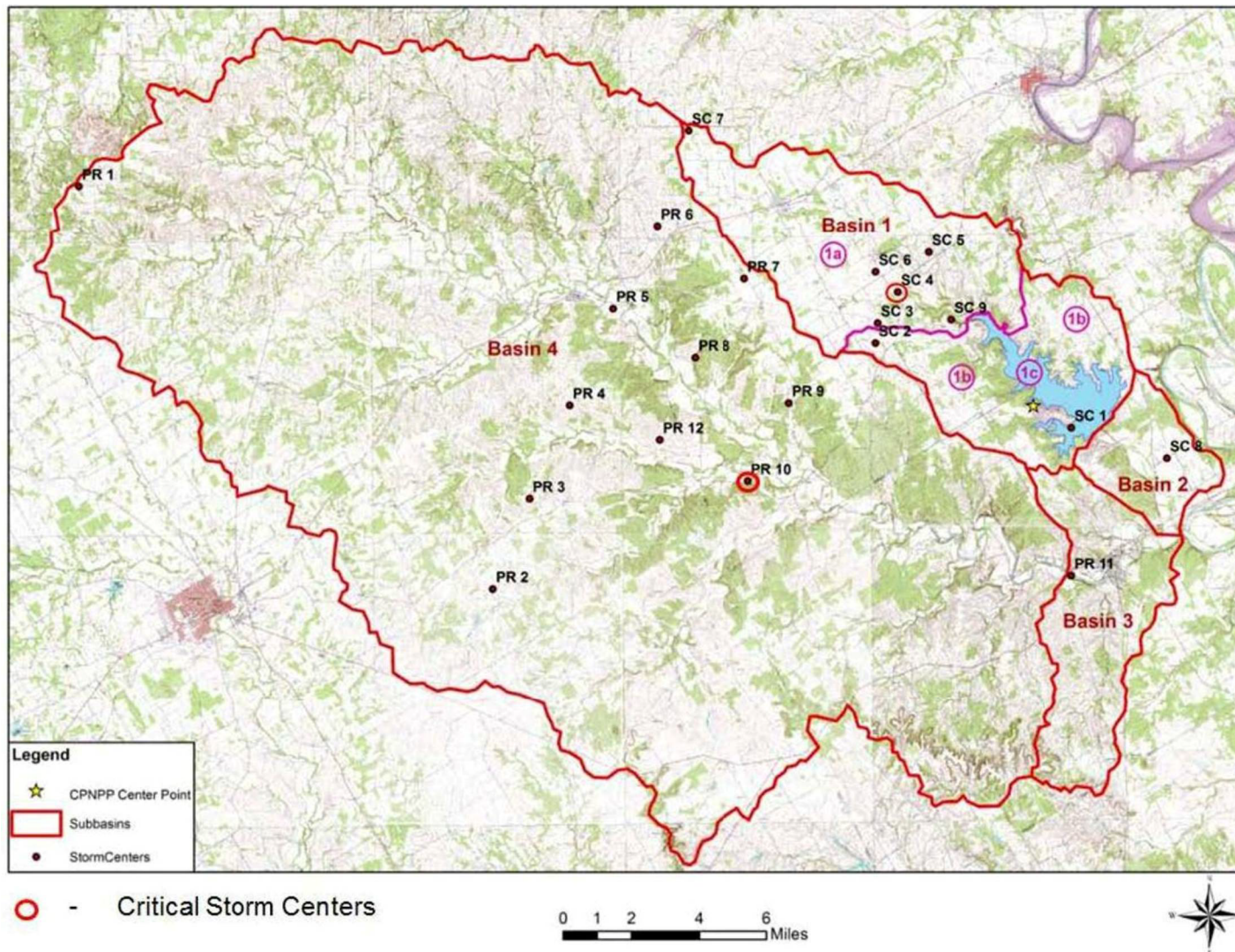
Figure 2.4.3-202 Watershed Sub-basins and Storm Centers
