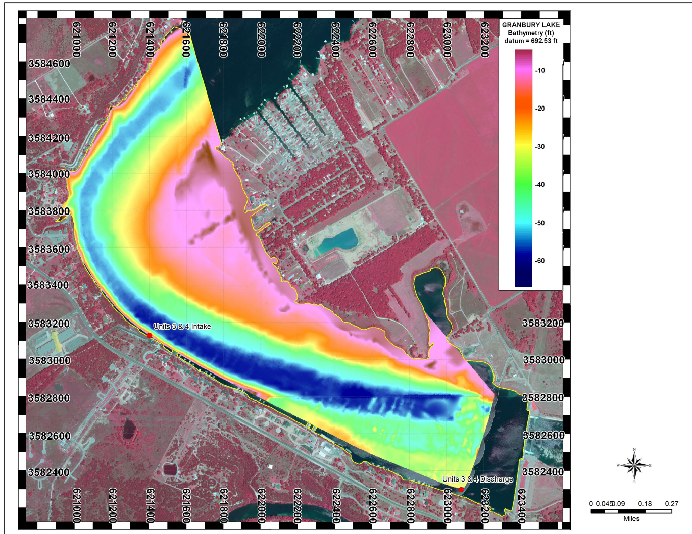
Figure 2.4.1-205 Lower Lake Granbury Bathymetric Survey Map
