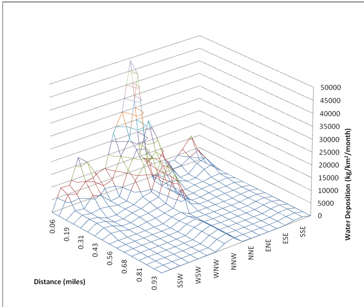
Figure 2.3-376 CPNPP Cooling Tower Water Deposition
