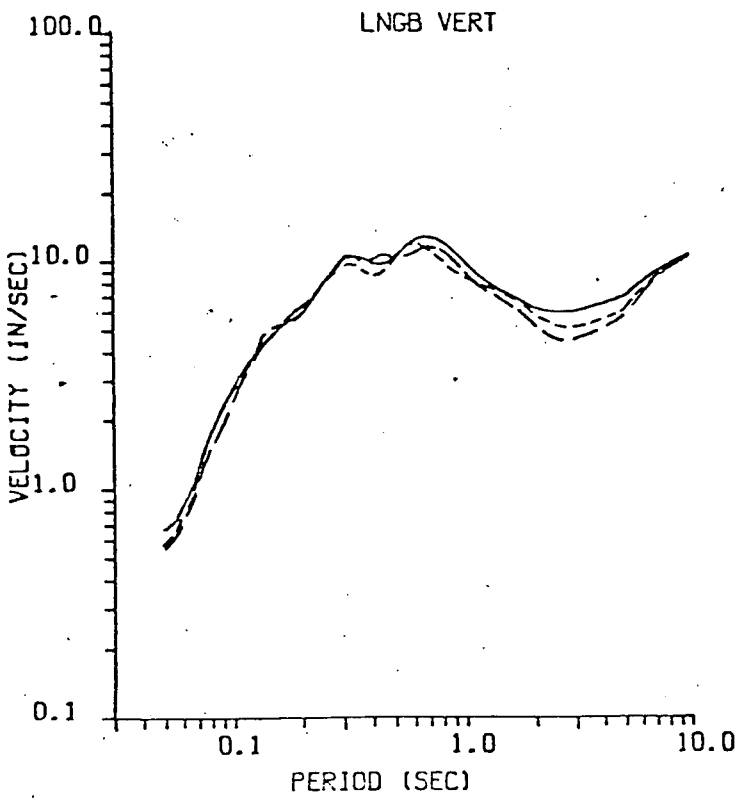
Figure 2-12. Comparison of the smoothed velocity response spectra computed from three earthquake models with fault tops at different depths.
