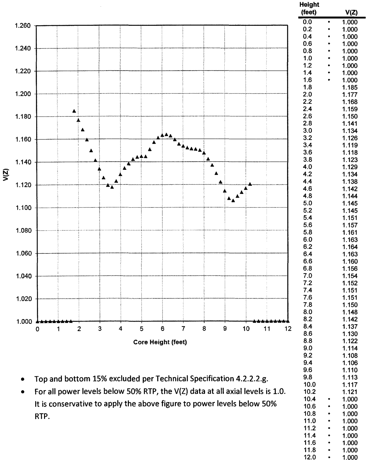
Figure 5 Cycle 19 V(Z) Versus Core Height 0 MWD/MTU ≤ burnup < 15000 MWD/MTU
