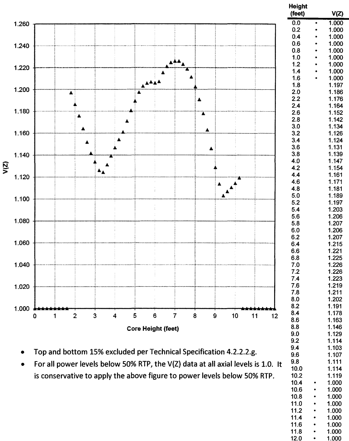
Figure 6 Cycle 19 V(Z) Versus Core Height 15000 MWD/MTU ≤ burnup ≤ 20610 MWD/MTU
