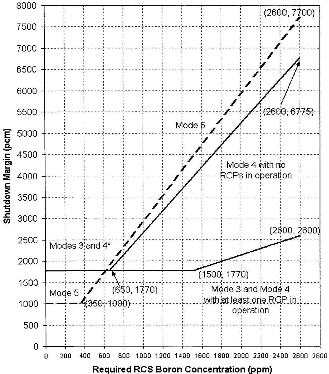
Figure 1 Shutdown Margin Versus RCS Boron Concentration Modes 3, 4, and 5/Drained
