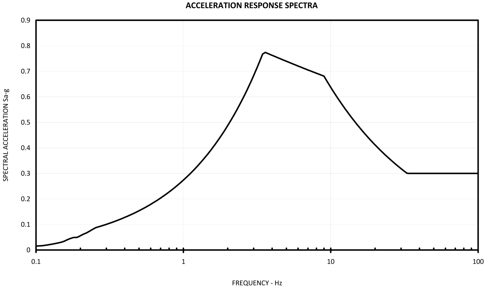
Figure 3.7-52 Service Building Vertical Input Motion for II/I Design (7% Damping)
