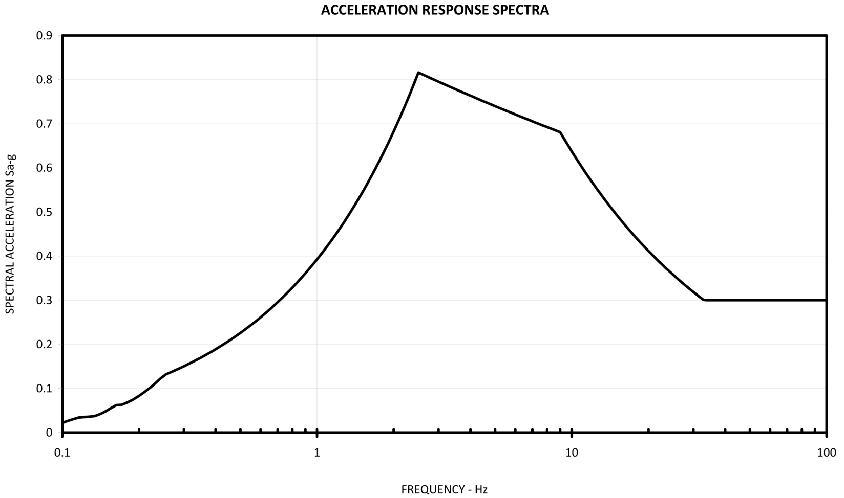
Figure 3.7-50 Service Building North-South Input Motion for II/I Design (7% Damping)
