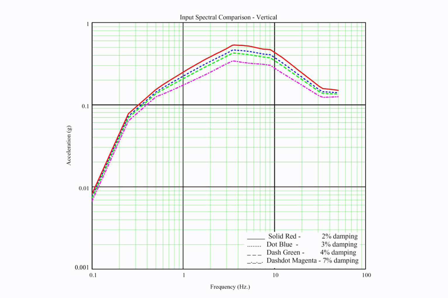
Figure 3.7-2b Plots of 2%, 3%, 4% and 7% Damped Input Response Spectrum – Vertical Direction
