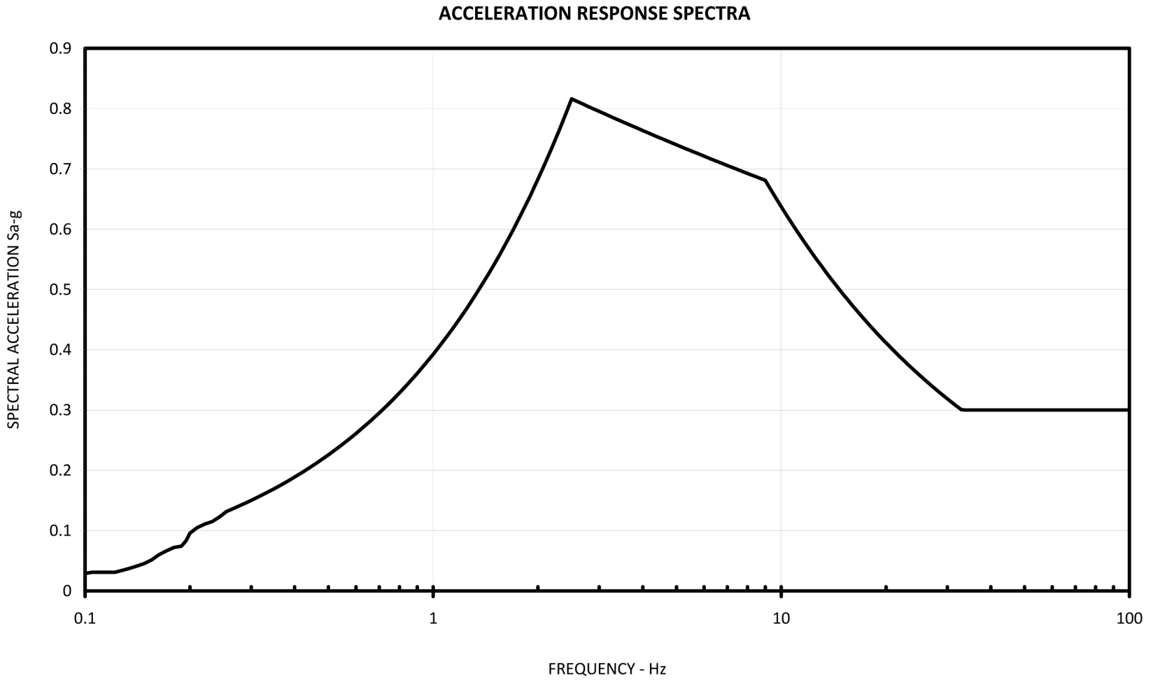
Figure 3.7-51 Service Building East-West Input Motion for II/I Design (7% Damping)
