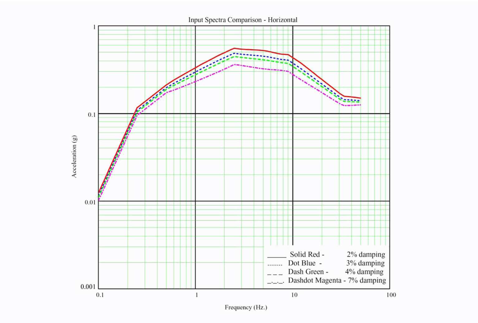
Figure 3.7-1b Plots of 2%, 3%, 4% and 7% Damped Input Response Spectrum – Horizontal Direction
