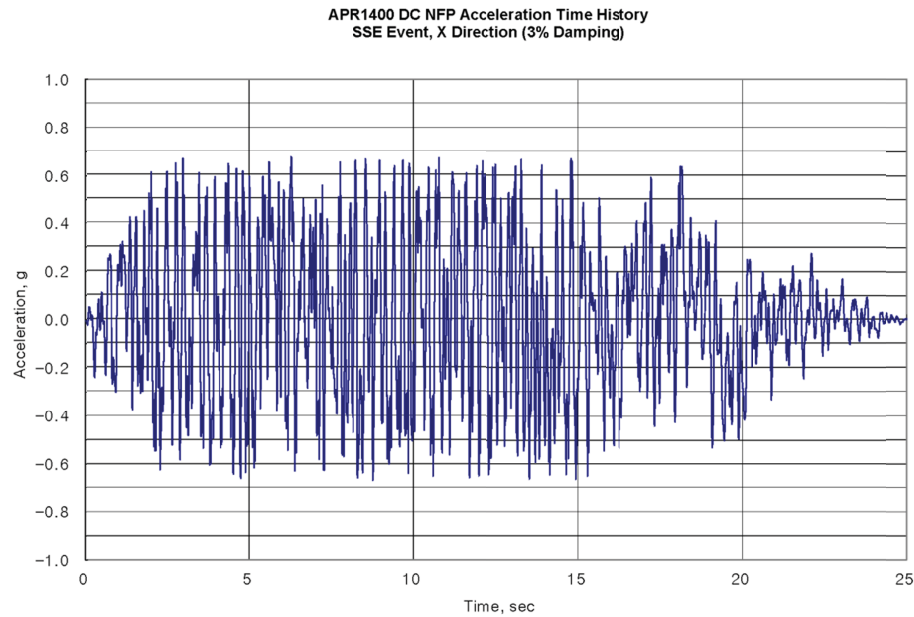
Figure A.3.4 137'-6" Acceleration-Time History Graph (3% Damping, E-W Direction)
