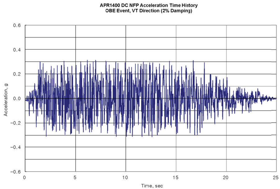
Figure A.3.3 137'-6" Acceleration-Time History Graph (2% Damping, Vertical Direction)
