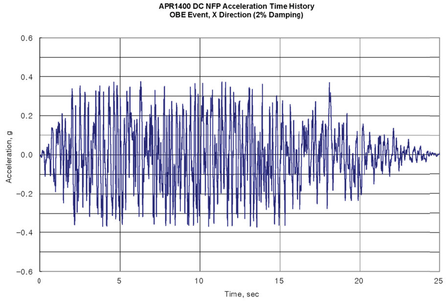
Figure A.3.1 137'-6" Acceleration-Time History Graph (2% Damping, E-W Direction)
