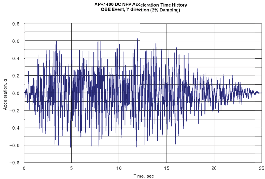
Figure A.3.2 137'-6" Acceleration-Time History Graph (2% Damping, N-S Direction)
