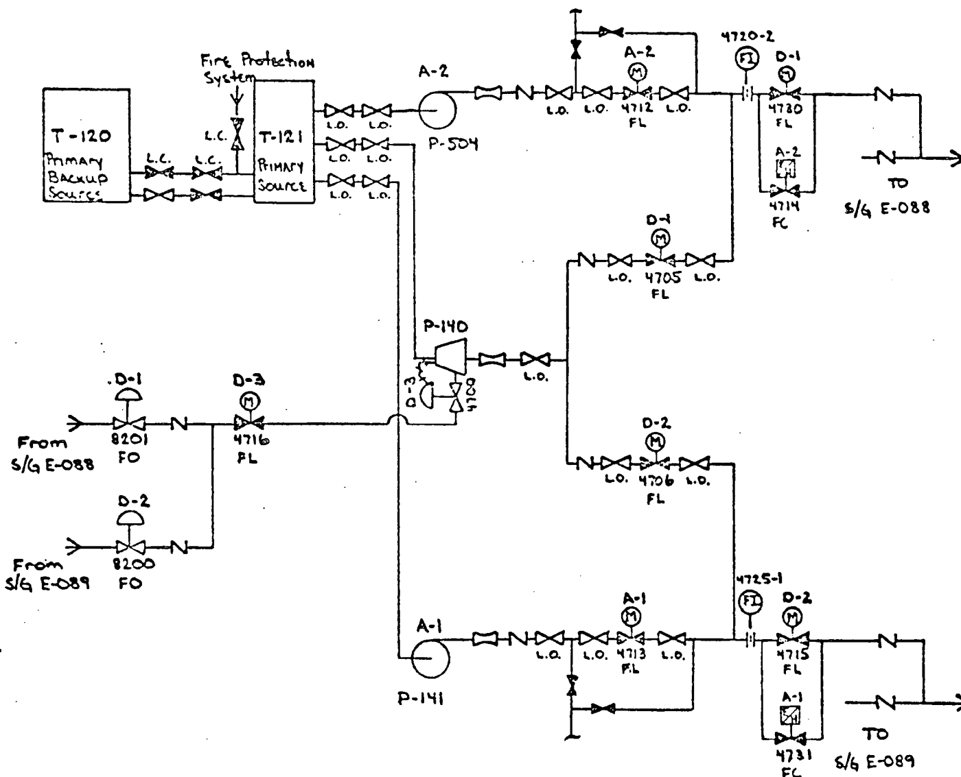
AUXILIARY FEEDWATER SYSTEM SONGS 213
