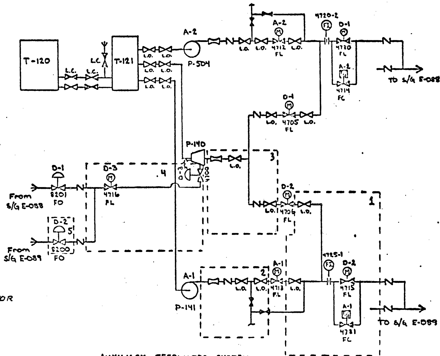
AUXILIARY FEEDWATER SYSTEM
