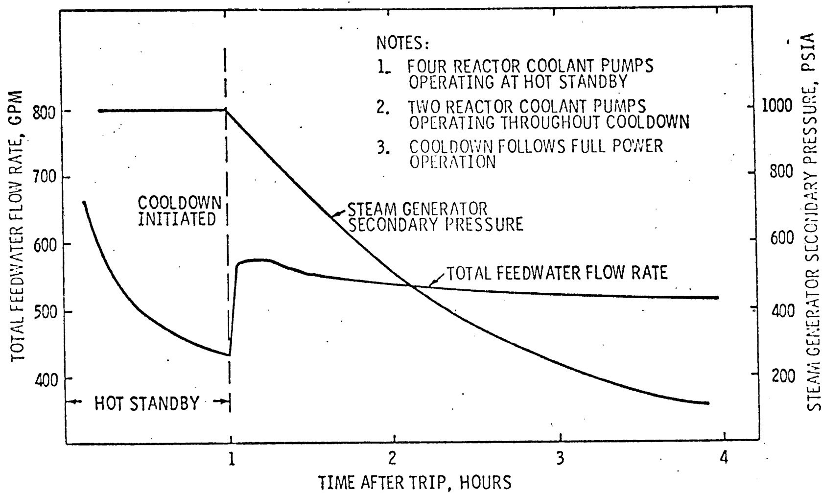
Figure 2-4 TYPICAL COOLDOWN
