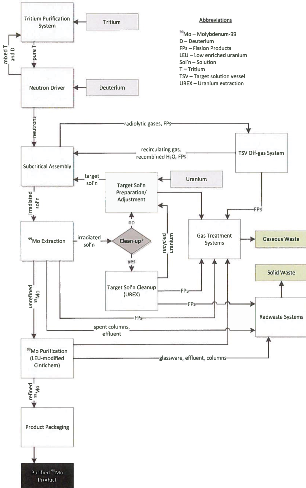
Figure 19.2.2-1 – Isotope Production System High-Level Flow Diagram
