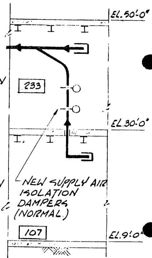
SECTION-C.
