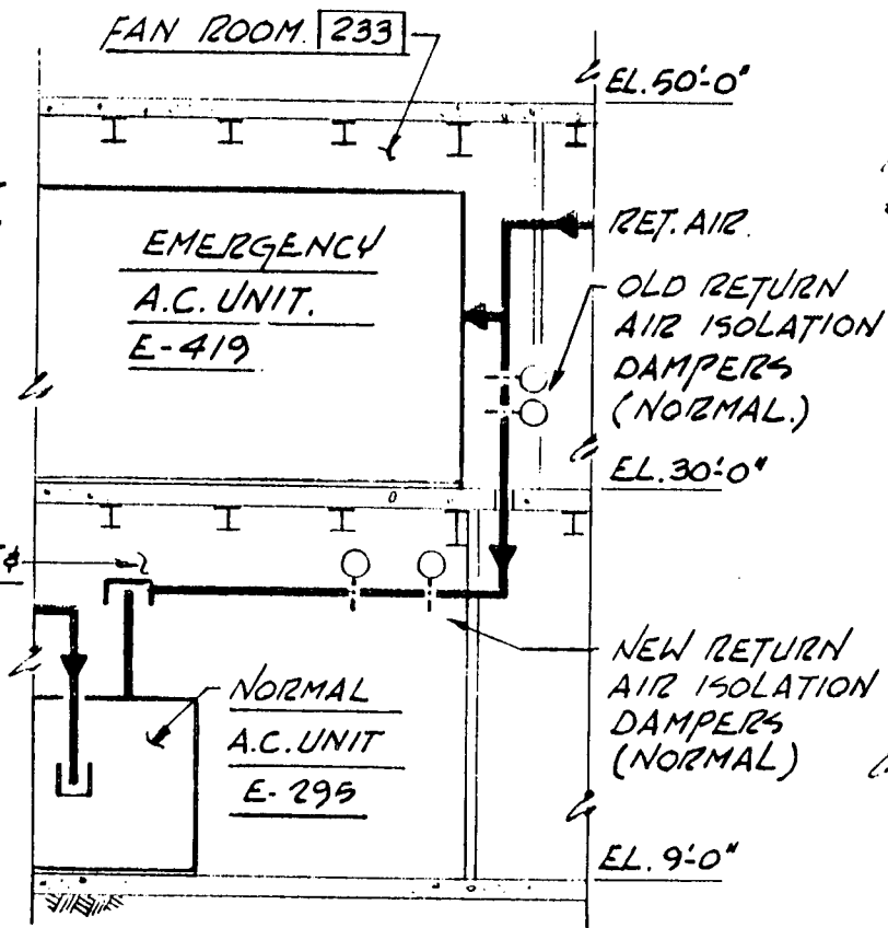
SECTION-B
