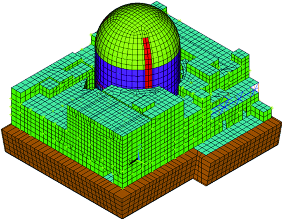
Figure 6-4. SASSI 3-D FEM of the Combined NI with Backfilled Soil
