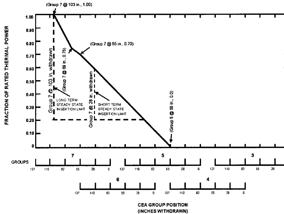
CEA GROUP POSITION (INCHES WITHDRAWN) FIGURE 3.1-2 CEA Insertion Limits vs. THERMAL POWER (4 Reactor Coolant Pumps Operating)
