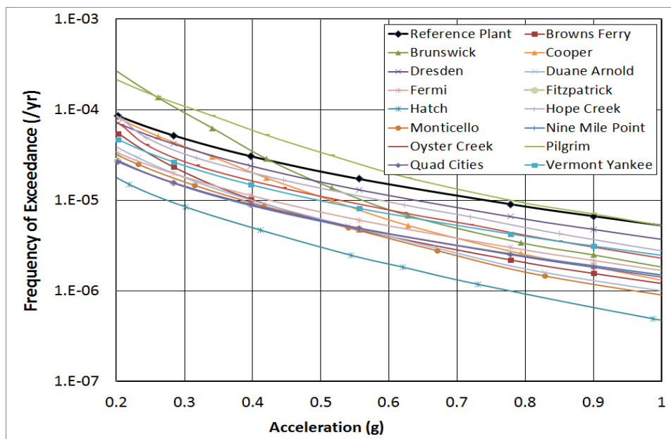
Figure 4 Comparison of annual PGA exceedance frequencies for U.S. Mark I reactors (USGS 2008 model) (rock hazard curves)
