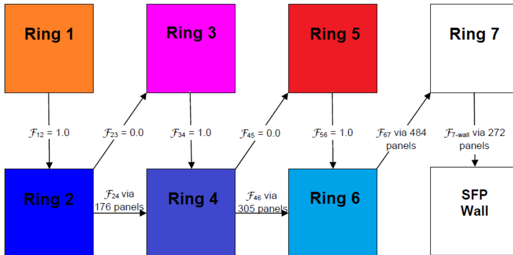
Figure 45 MELCOR radial radiative coupling scheme
