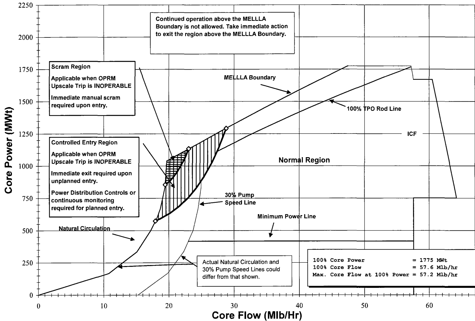
Figure 5 Monticello Cycle 27 Power/Flow Map
