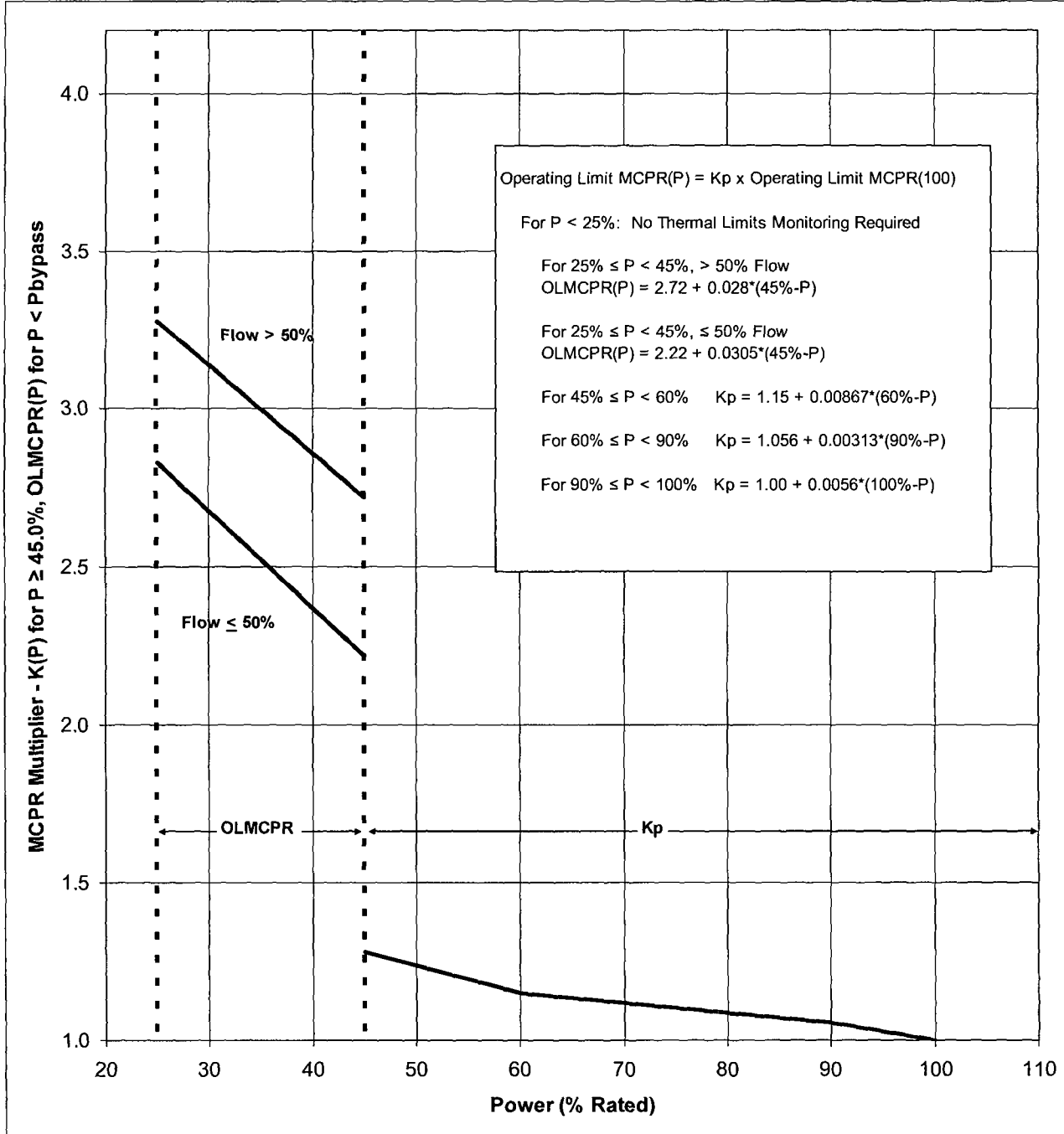
Figure 3 Monticello Cycle 27 Power Dependent K(P) / MCPR(P) Limits
