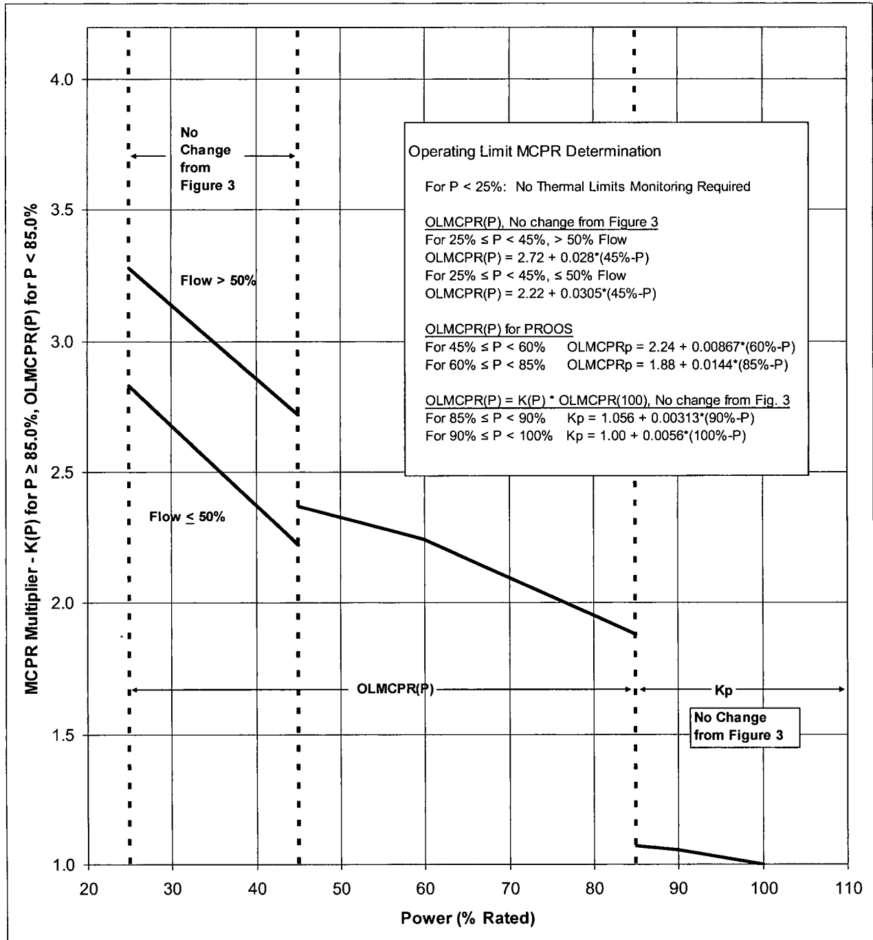
Figure 8 Monticello Cycle 27 Power Dependent K(P) and MCPR(P) Limits for Pressure Regulator Out of Service (PROOS) for CLTP Conditions
