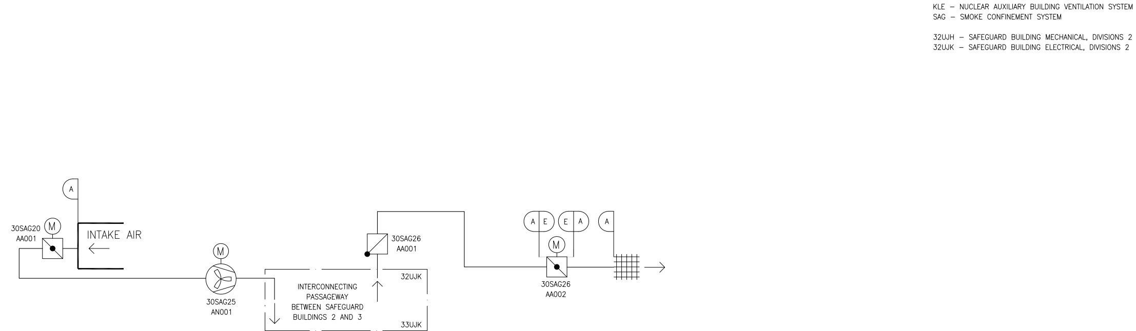
Figure 9.4.13-1—Smoke Confinement System
