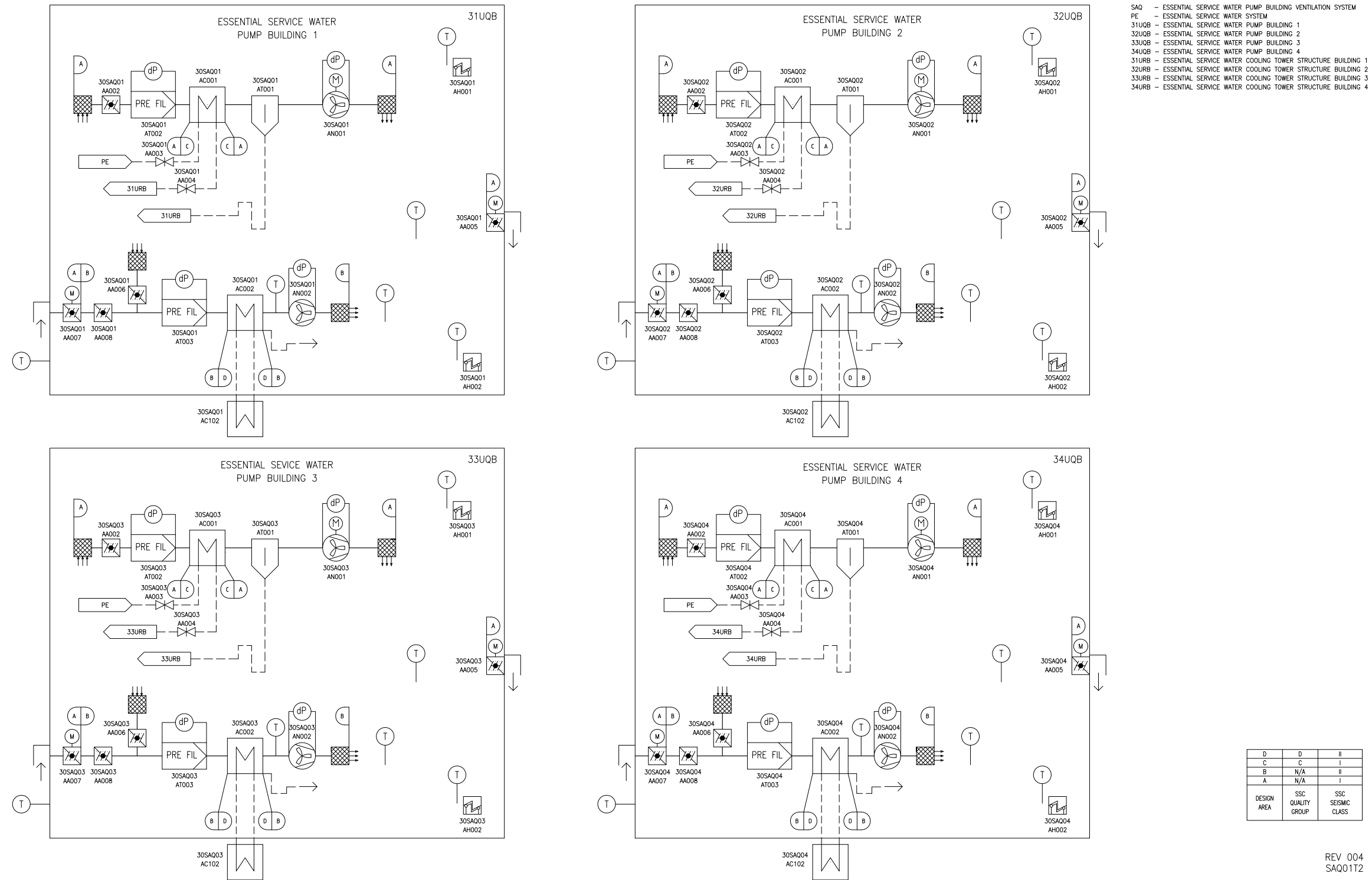
Figure 9.4.11-1—Essential Service Water Pump Building Ventilation System
