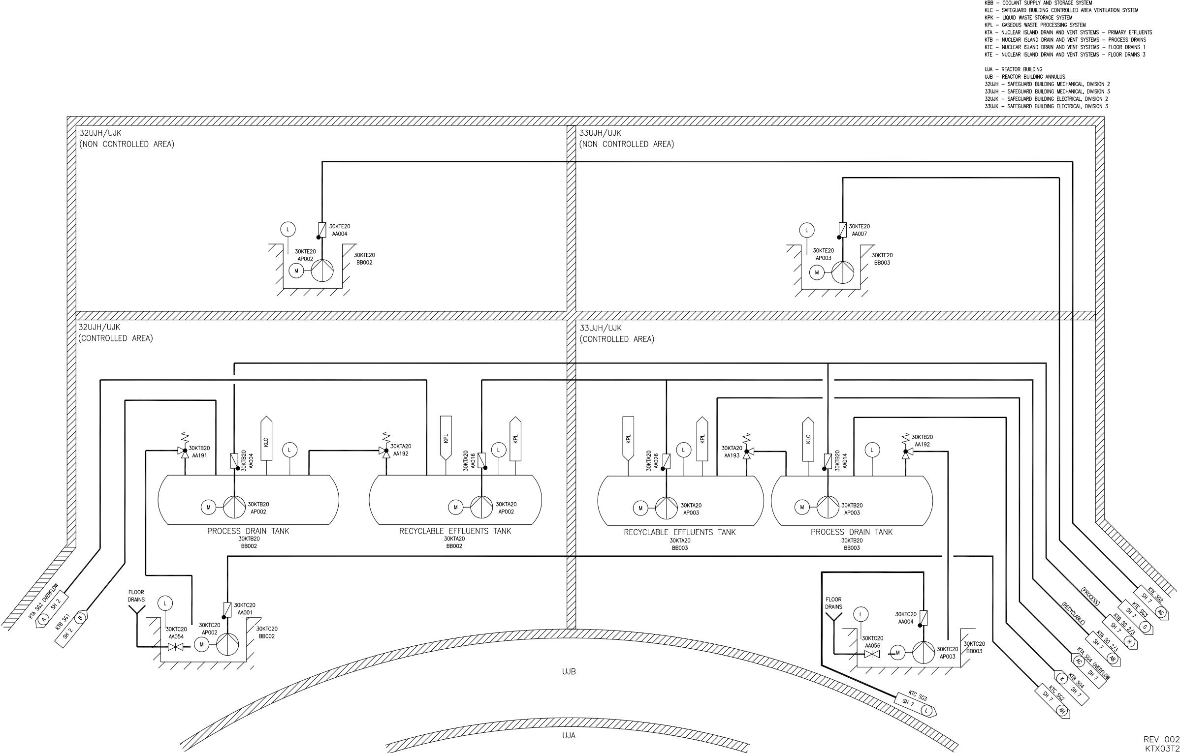
Figure 9.3.3-1—Nuclear Island Drain and Vent System Sheet 3 of 9
