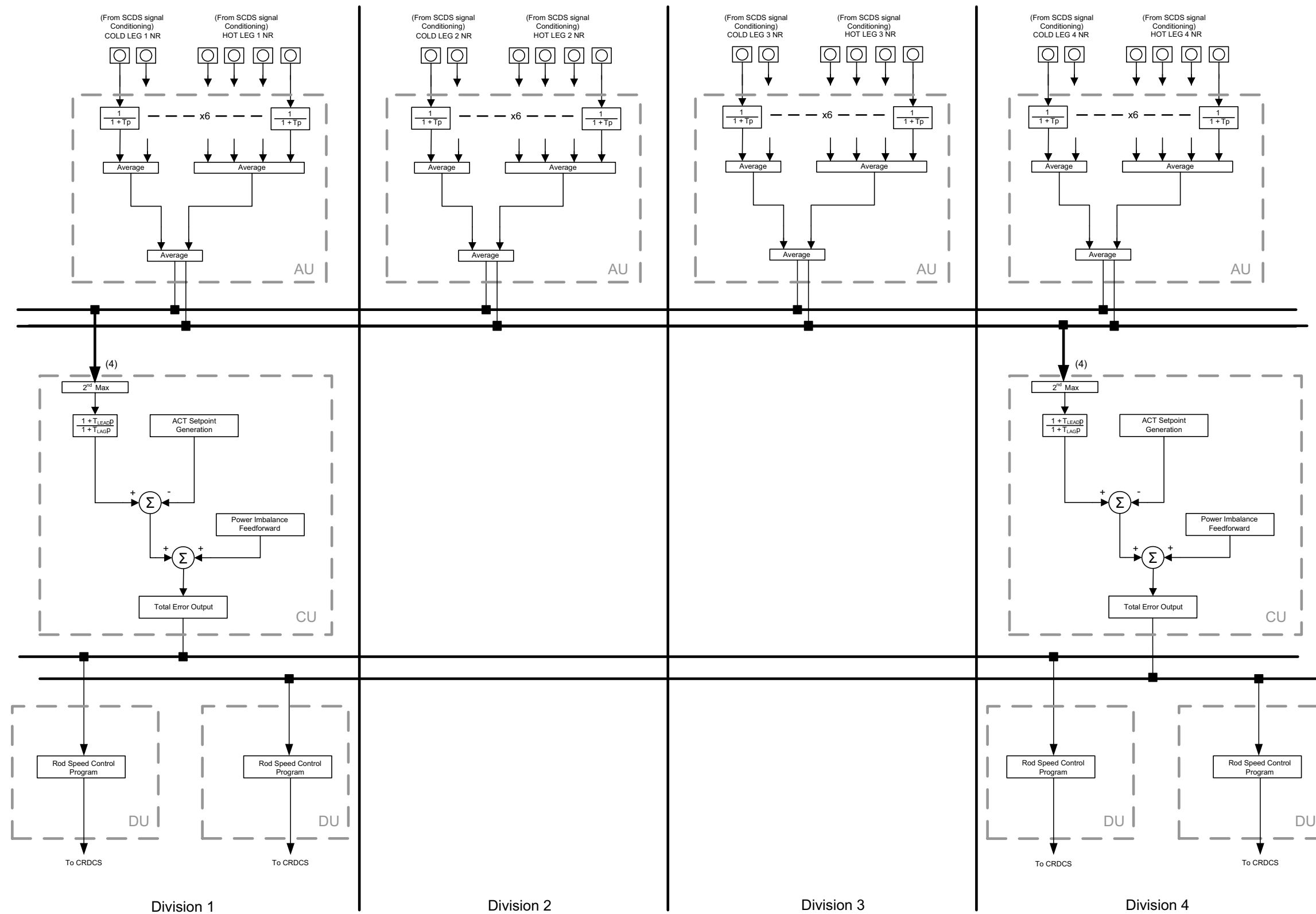
Figure 7.7-6—Signal Flow from SCDS through CU
