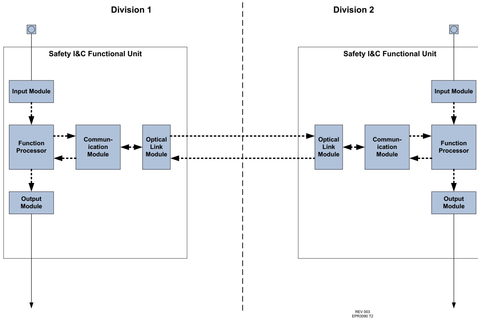
Figure 7.1-19—Implementation of Independence Between Redundant Divisions
