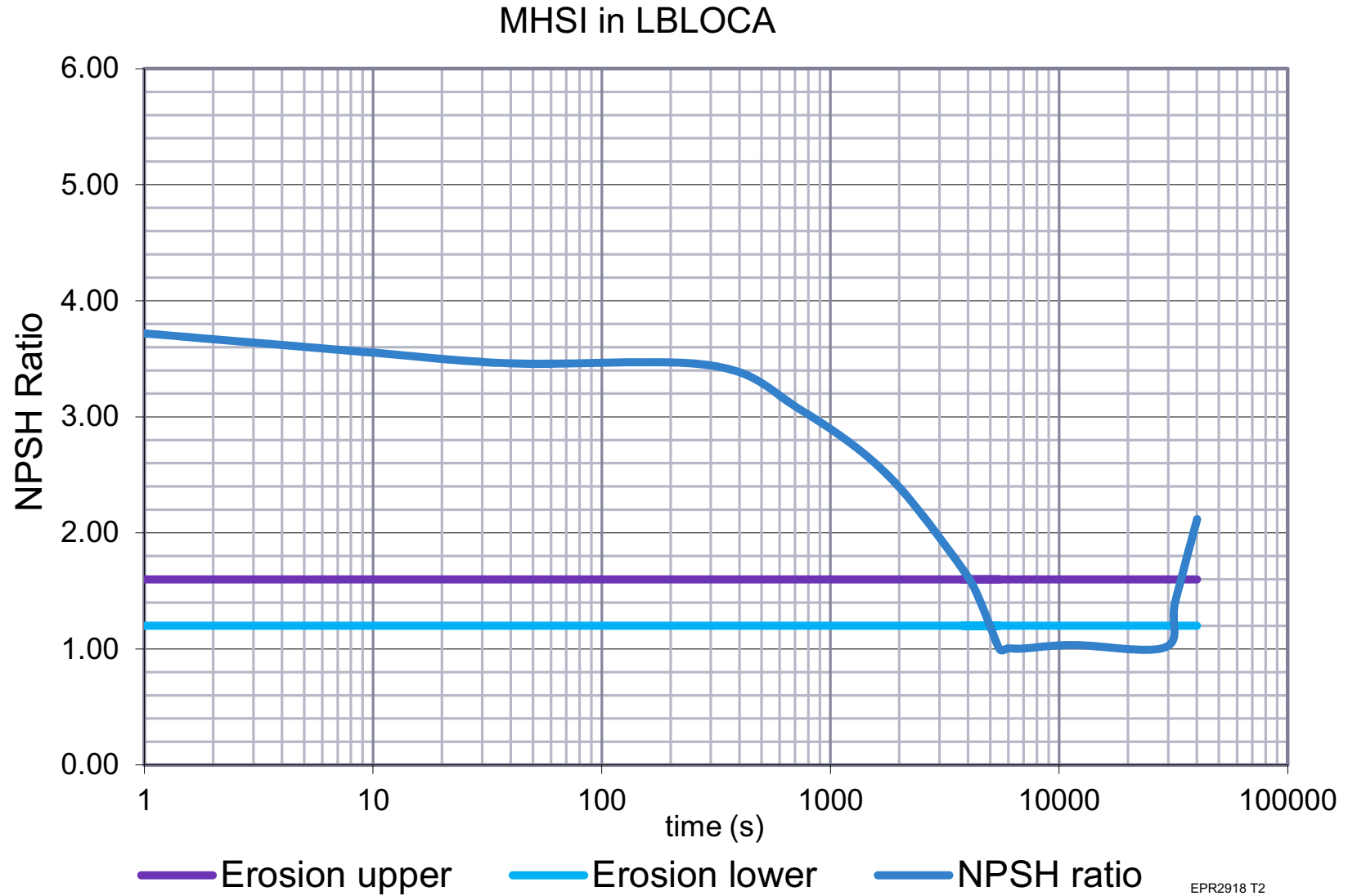
Figure 6.3-11—MHSI in LB LOCA - Cavitation Erosion
