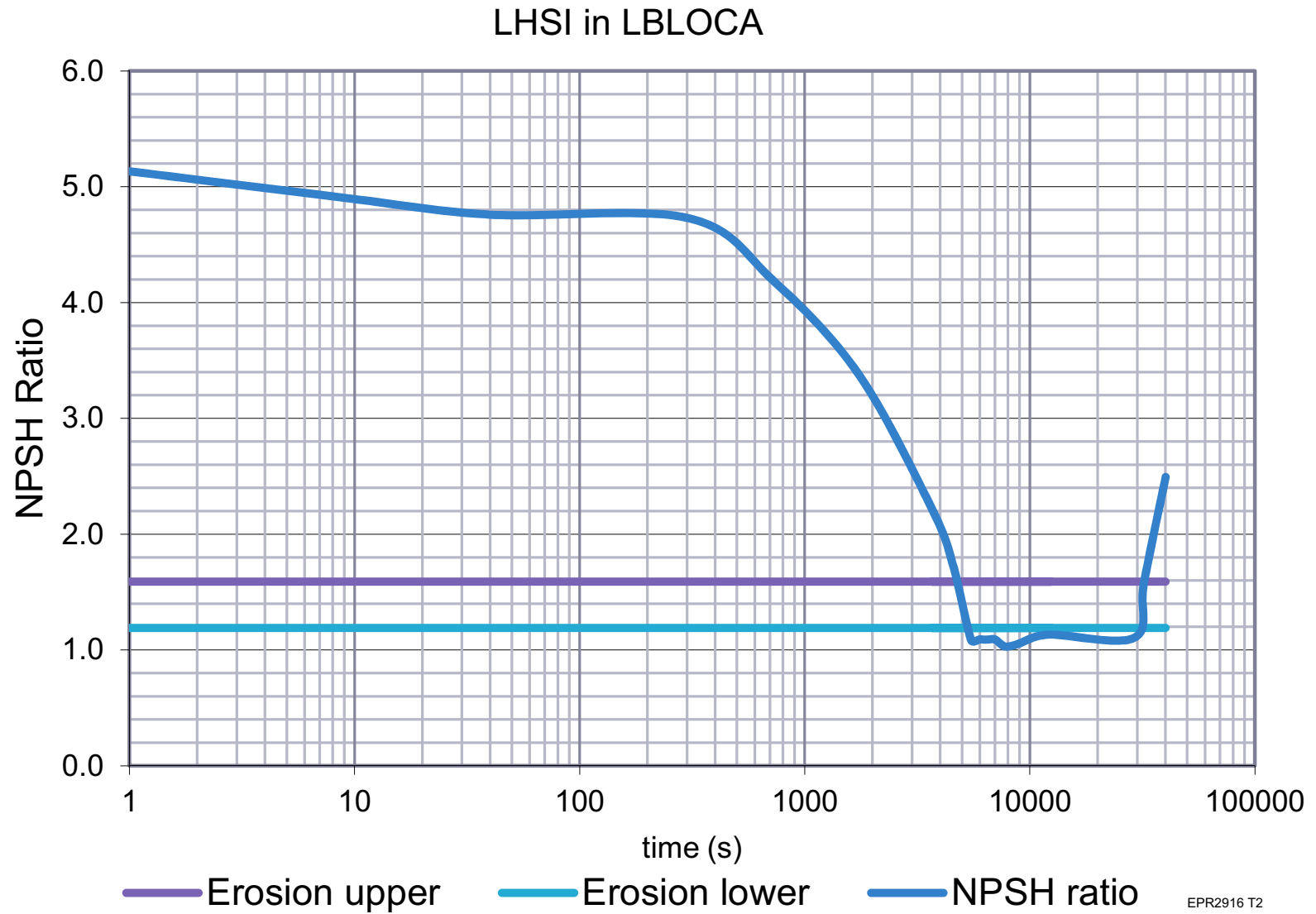
Figure 6.3-10—LHSI in LBLOCA - Cavitation Erosion
