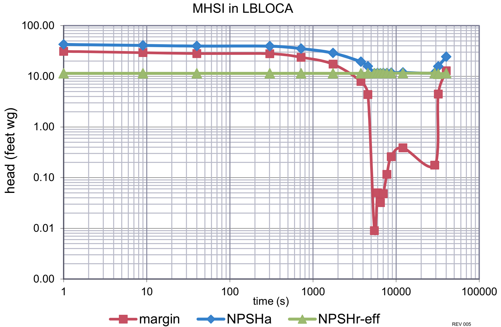
Figure 6.3-9—MHSI in LBLOCA
