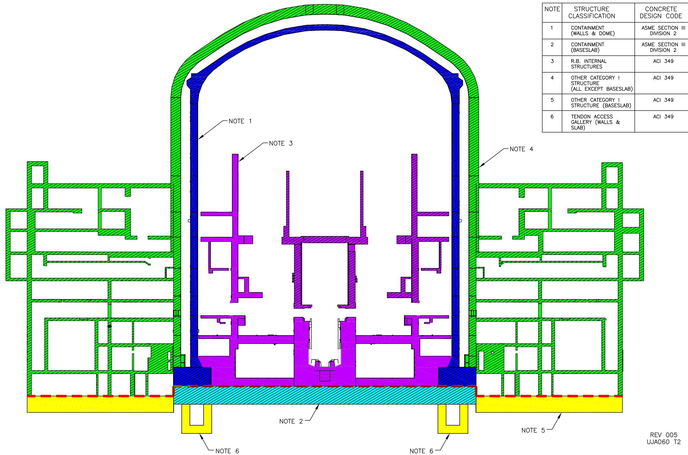
Figure 3.8-118—Jurisdictional Boundaries for the Design of Concrete Structures of the U.S. EPR Common Basemat Structure
