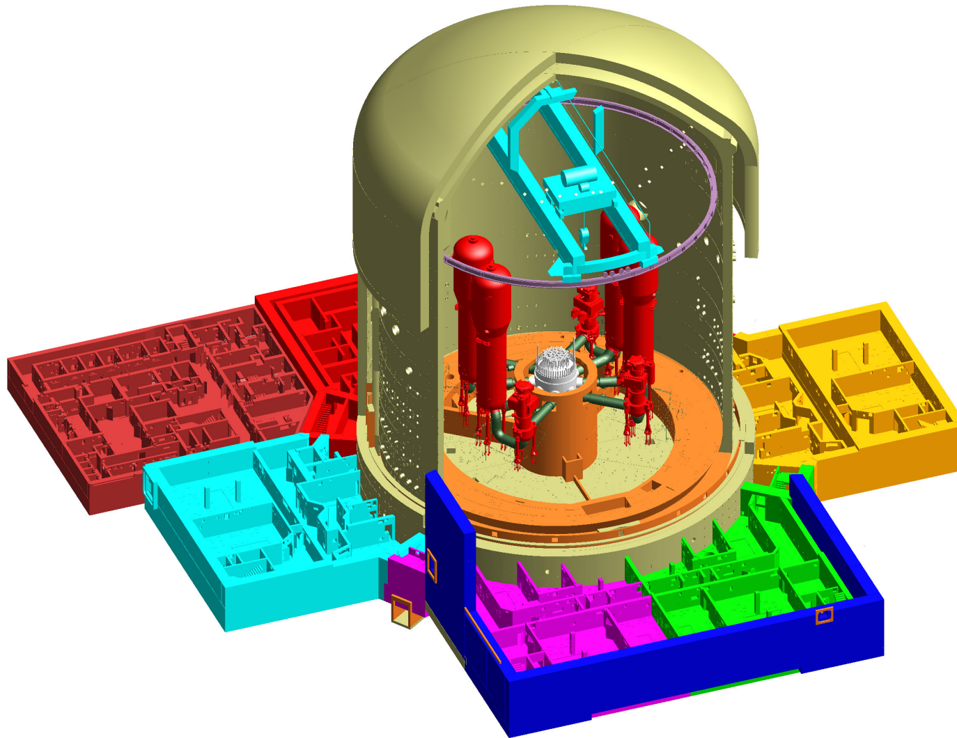
Figure 1.2-2—U.S. EPR Cutaway
