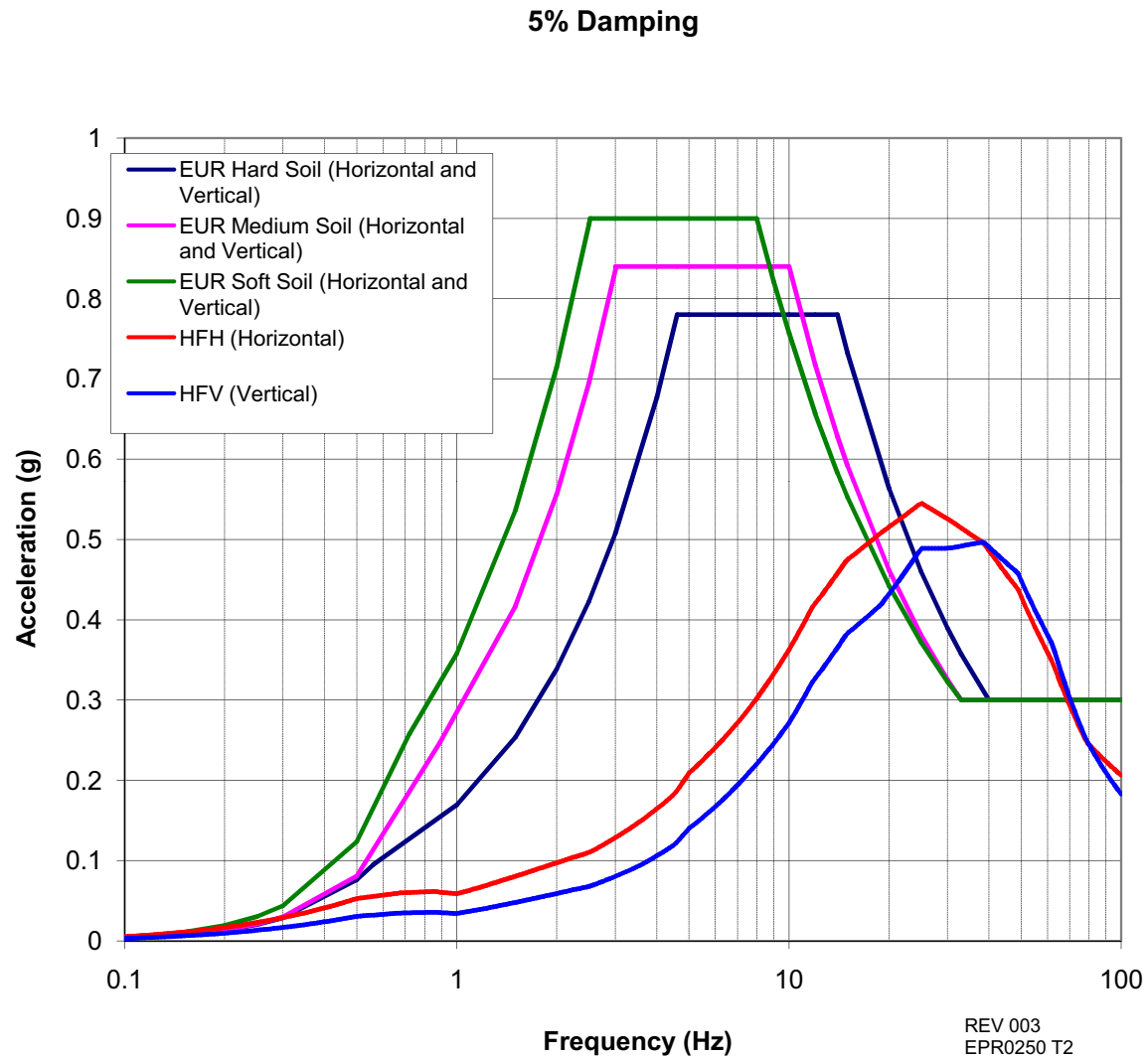
Figure 5.0-1—Design Response Spectra for EUR (Hard, Medium and Soft Sites) and HF Control Motions
