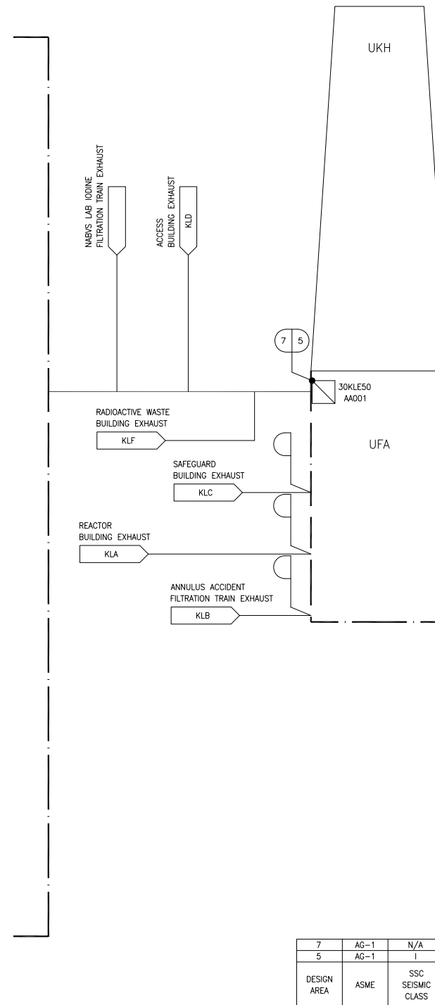
Figure 2.6.5-1—Nuclear Auxiliary Building Exhaust Filtration Trains Subsystem Functional Arrangement
