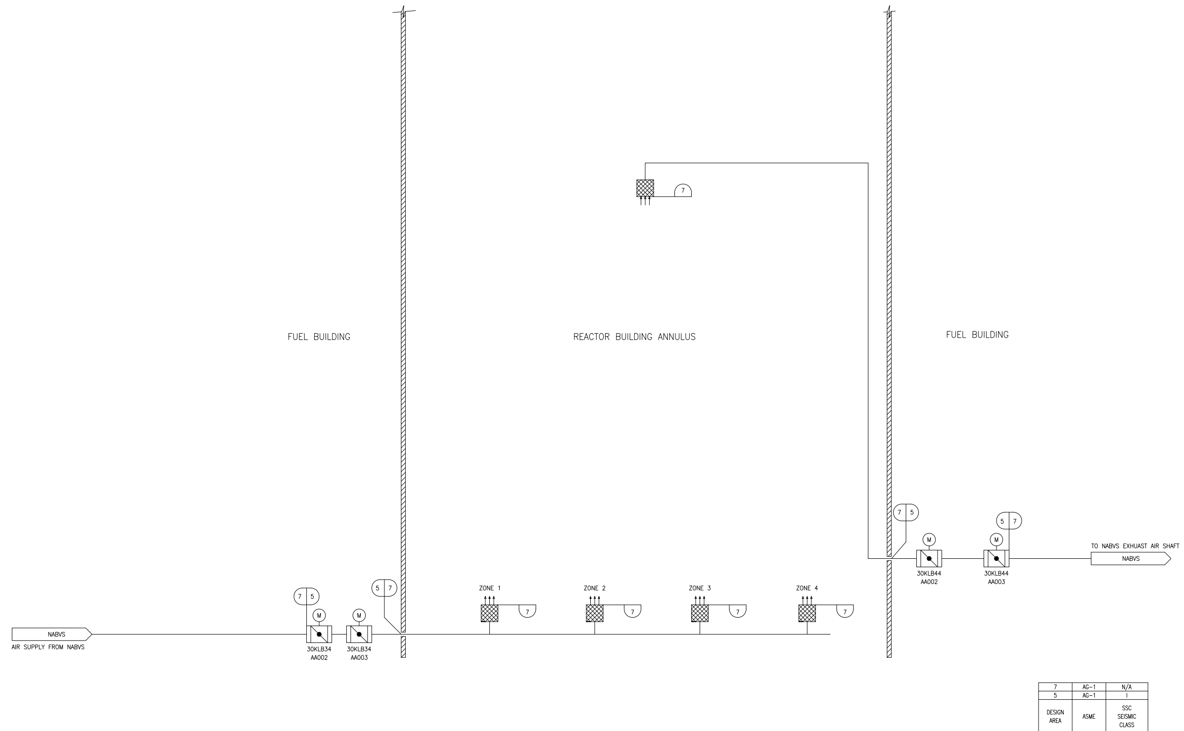
Figure 2.6.3-1—Annulus Ventilation System Normal Operation Train Functional Arrangement
