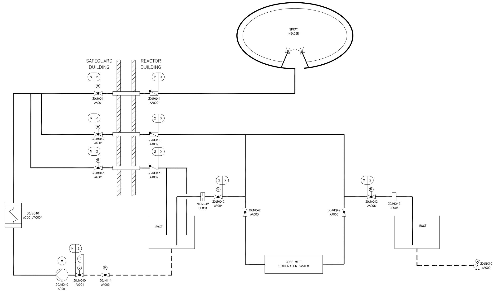
Figure 2.3.3-1—Severe Accident Heat Removal System Functional Arrangement
