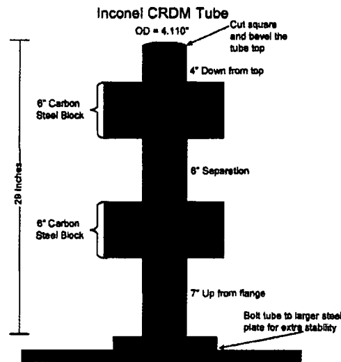
Figure 1. Assembled CRDM interference fit mock-up specimen
