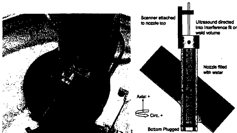
Figure 5 Left: Scanner on Calibration Specimen. Right: Inspection Schematic
