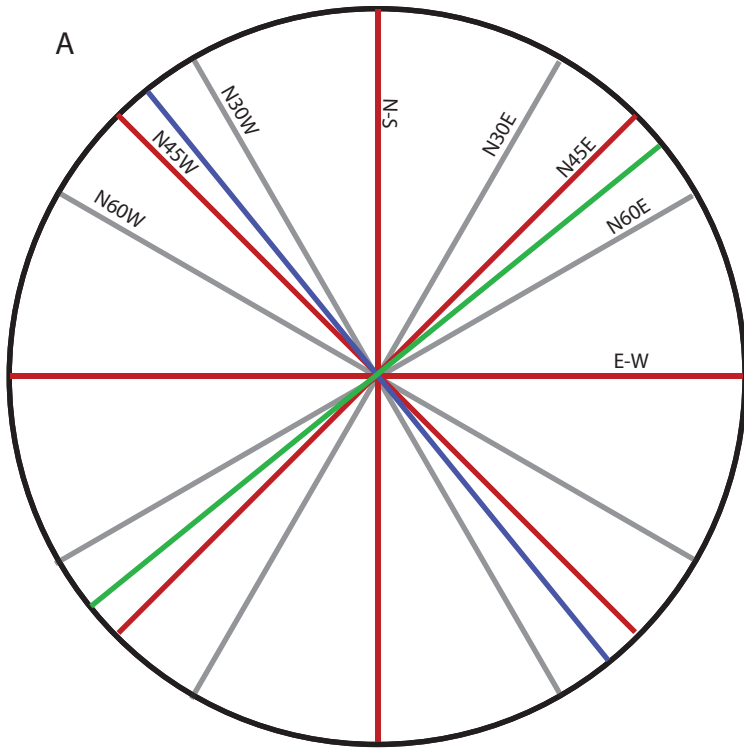
A: Joint orientations observed in Crystal River Unit No. 3 Excavation (no information on frequency or number of observations) (CR3 FSAR, 1973).
