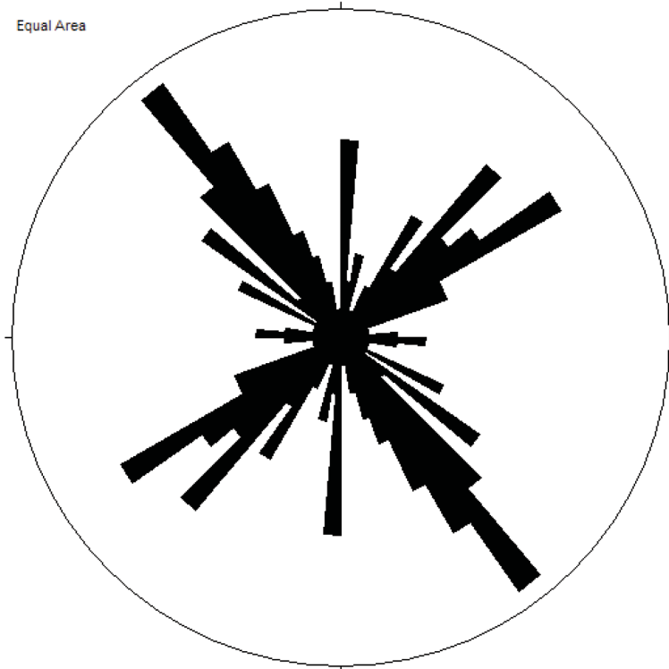
B: Rose diagram showing orientation and frequency of mapped lineaments within the site location (1-km [0.6-mi.] radius)
