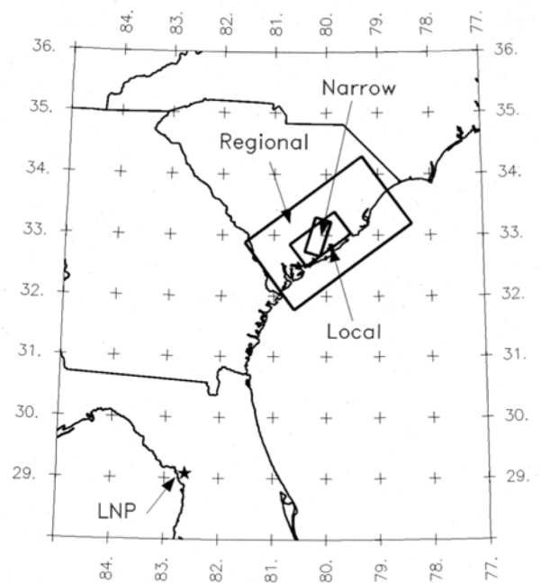
CEUS SSC Model, Charleston RLME Source
