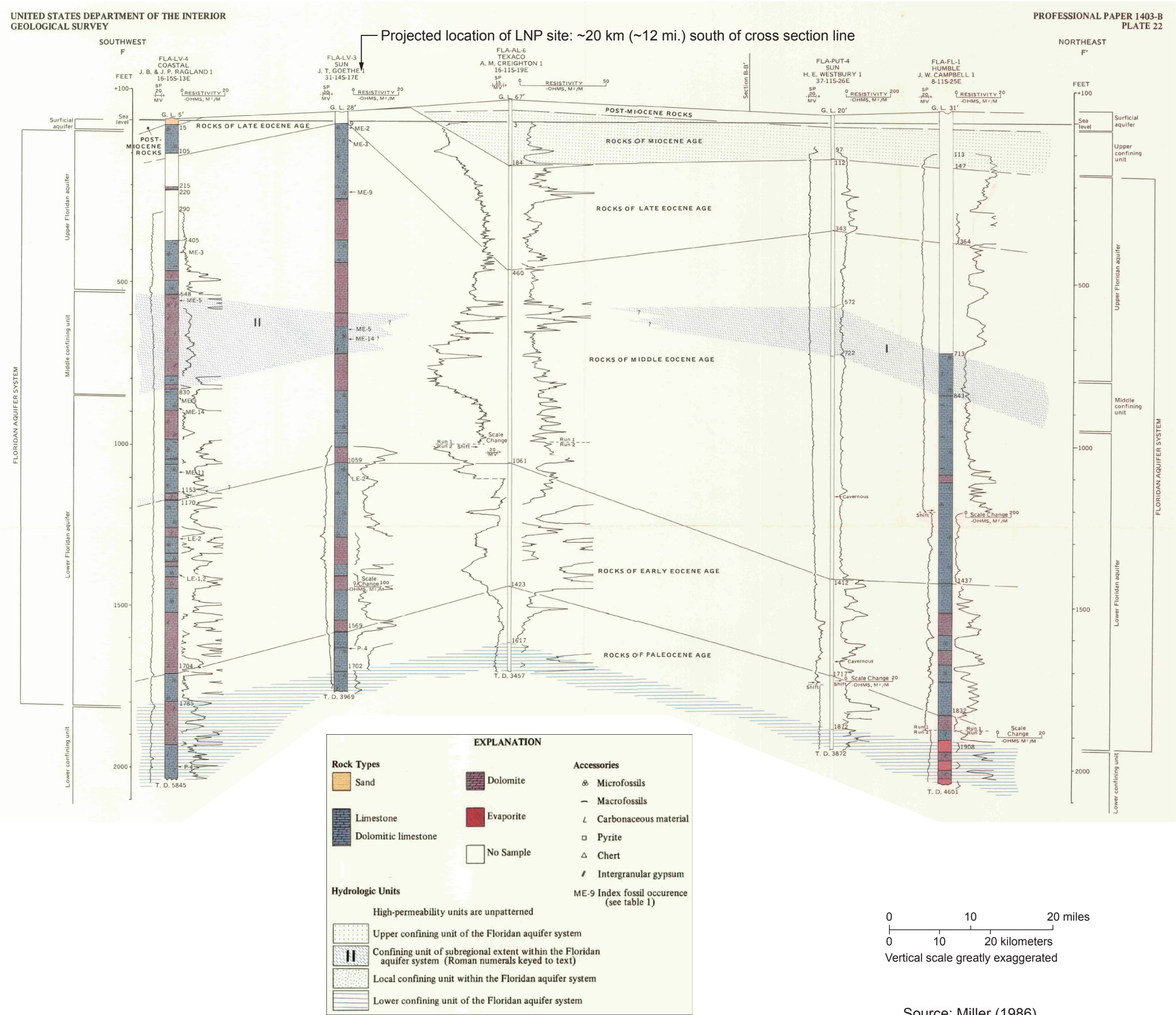
Duke Energy Florida Levy Nuclear Plant Units 1 and 2 Part 2, Final Safety Analysis Report Geohydrologic Cross Section F-F' from Levy County, Florida, to Flagler County, Florida FIGURE 2.5.1-217 Rev 6
