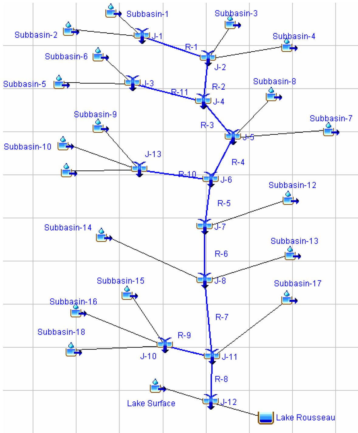
Duke Energy Florida Levy Nuclear Plant Units 1 and 2 Part 2, Final Safety Analysis Report Schematic of Basin Elements and their Connectivity FIGURE 2.4.3-214 Rev 6
