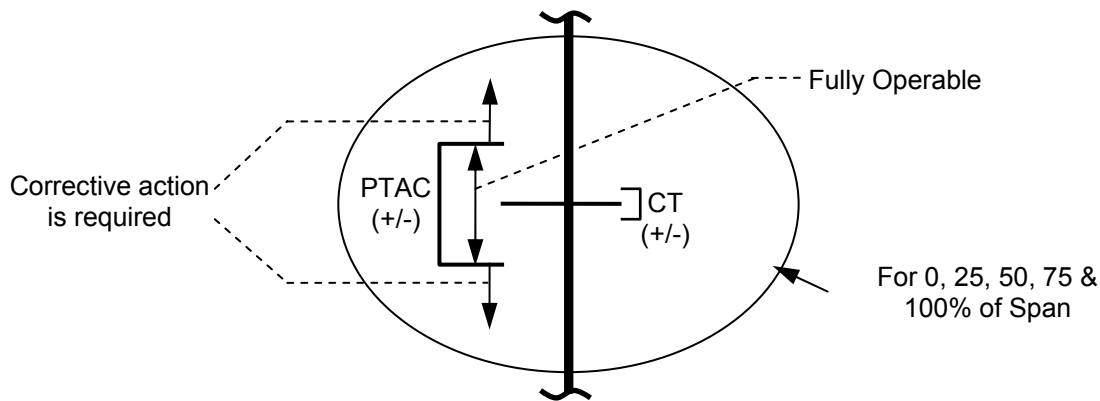
Figure 5-4 Channel Calibration on Analog Measurements
