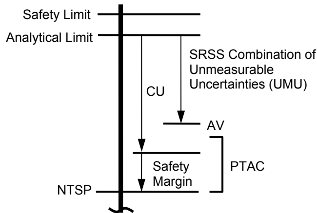
Figure 5-3 Relationship between AL and NTSP, AL and AV
