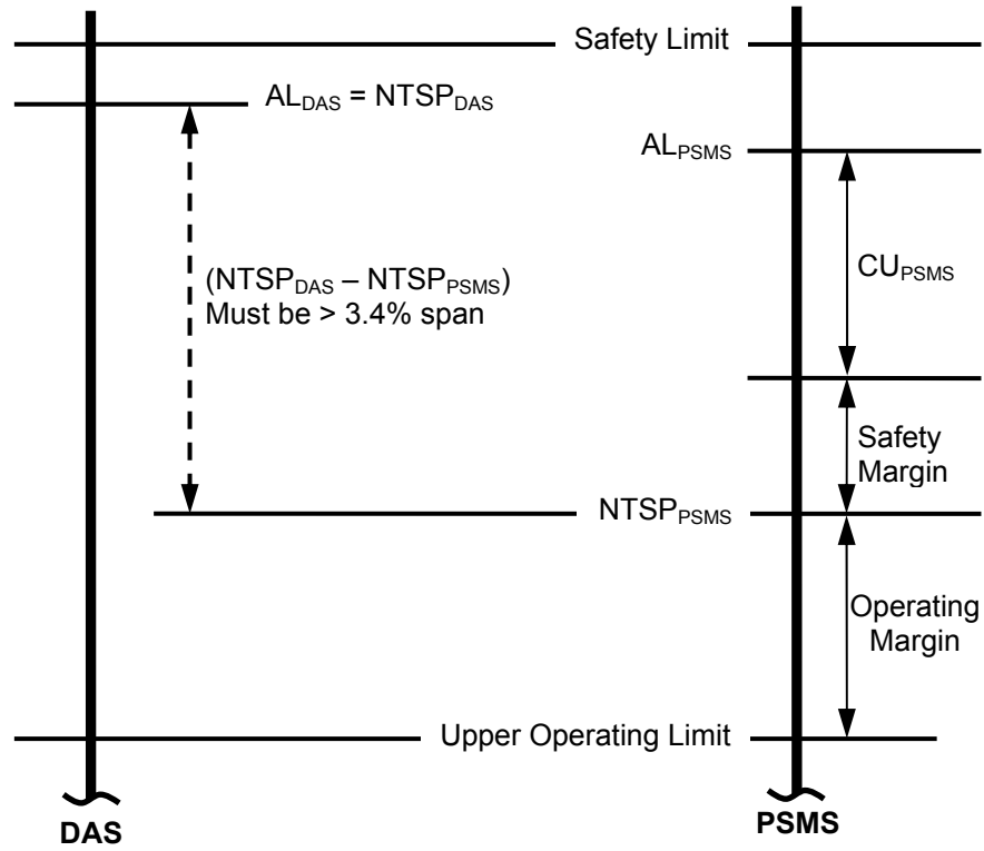
Figure 5-9 DAS vs PSMS Setpoints Relationship (Increasing Process)
