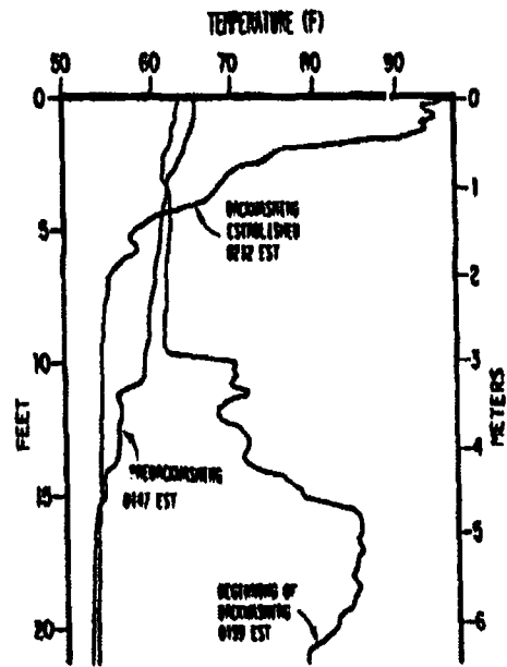
Fig. 8 Temperature profiles from Station 1 during the start of backwashing of the east circulating water pump on July 17, 1977.
