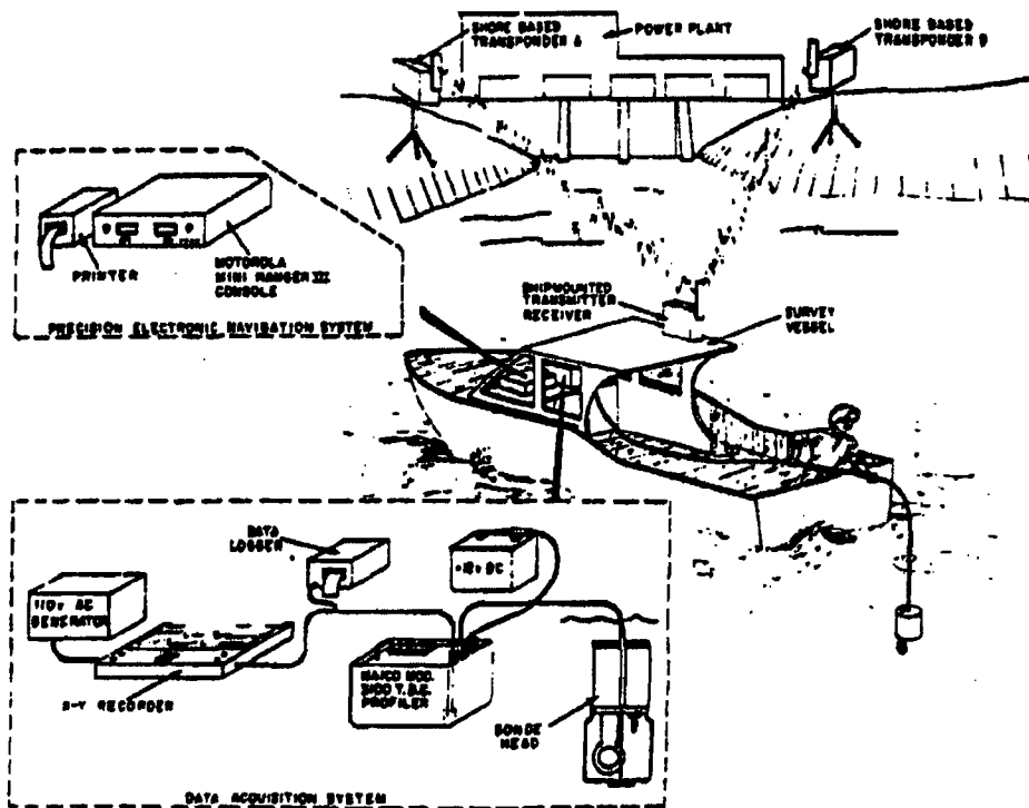
Fig. 2 Instrumentation set up for field surveys.
