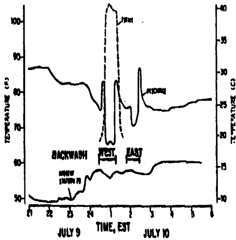
Fig. 3 Temperature monitor data from the west pump waterbox, the discharge canal and the ambient in situ unit at Station 28 during backwashing operations on July 9 and 10, 1977.
