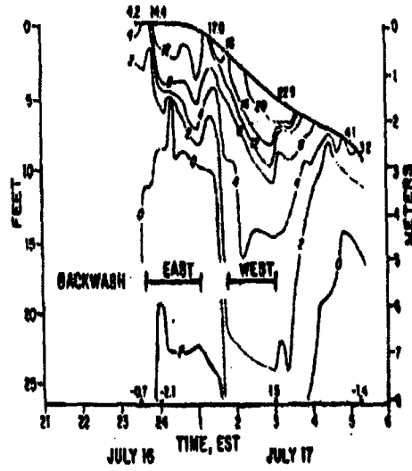
Fig. 7 Temperature data from an anchored survey boat at Station 6 on July 16 and 17, 1977 showing actual temperatures and corresponding \Delta T 's above ambient in degrees F.
