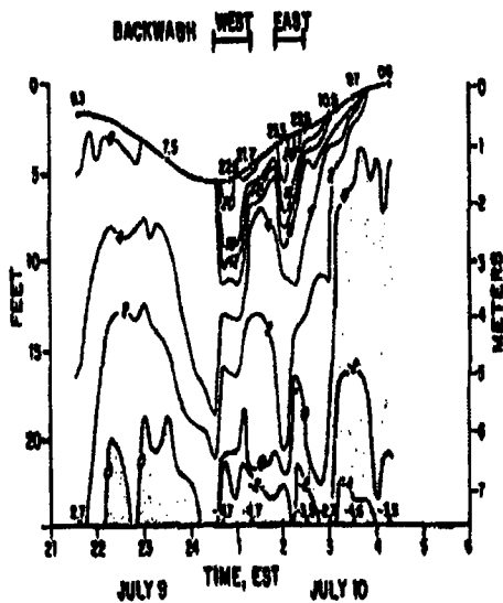
Fig. 5 Temperature data from an anchored survey boat at Station 6 on July 9 and 10, 1977 showing actual temperatures and corresponding \Delta T 's above ambient in degrees F.
