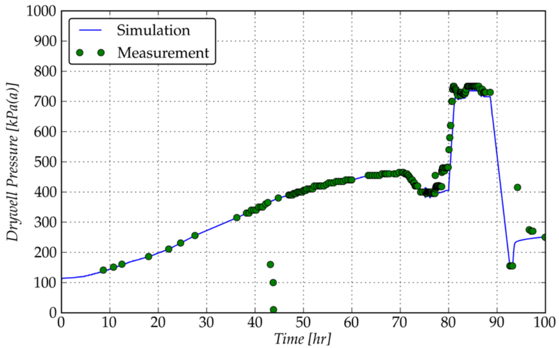
Figure 5-2: Simulation of Containment Pressure Response at 1F2 using MAAP5
