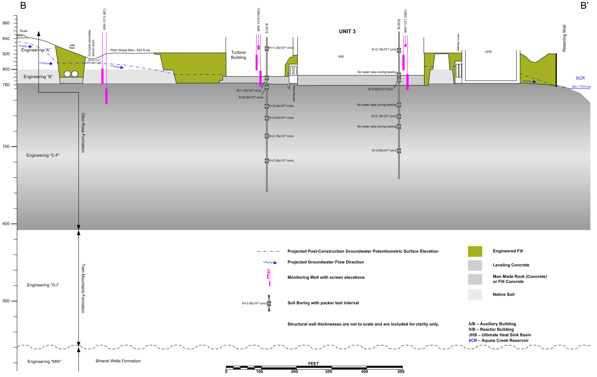
Figure 1-3 Cross-Section B-B'
