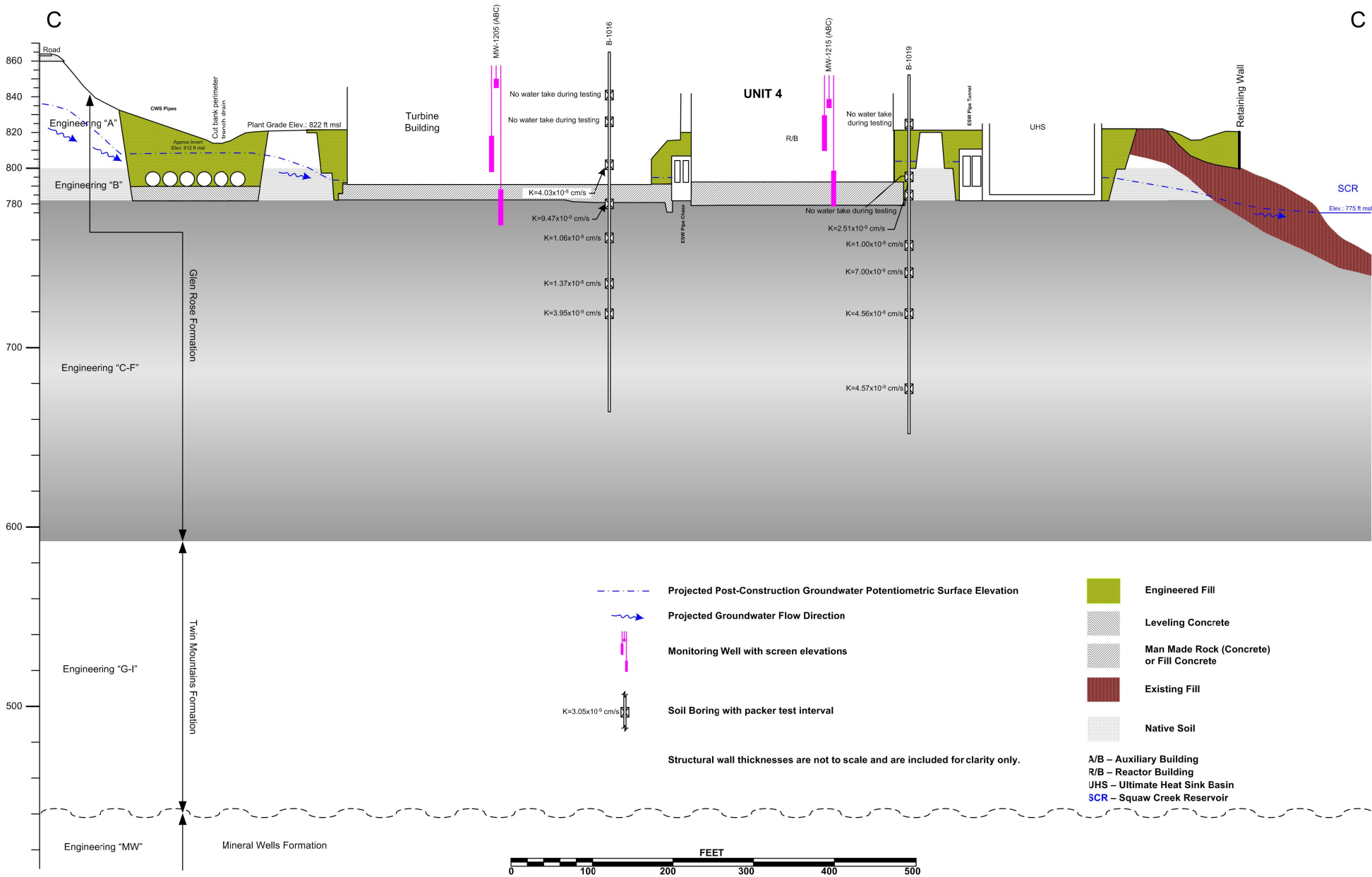
Figure 1-4 Cross-Section C-C'
