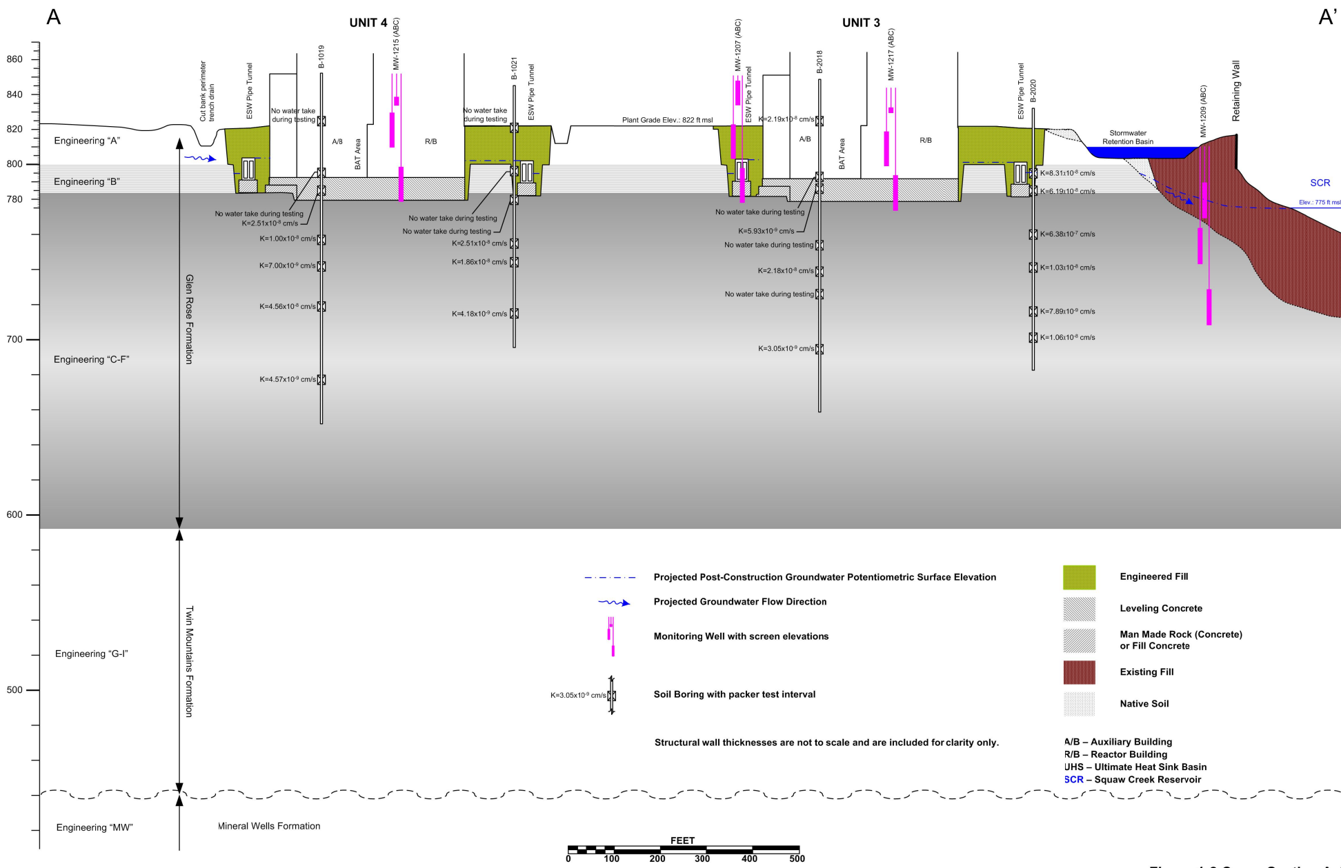
Figure 1-2 Cross-Section A-A'
