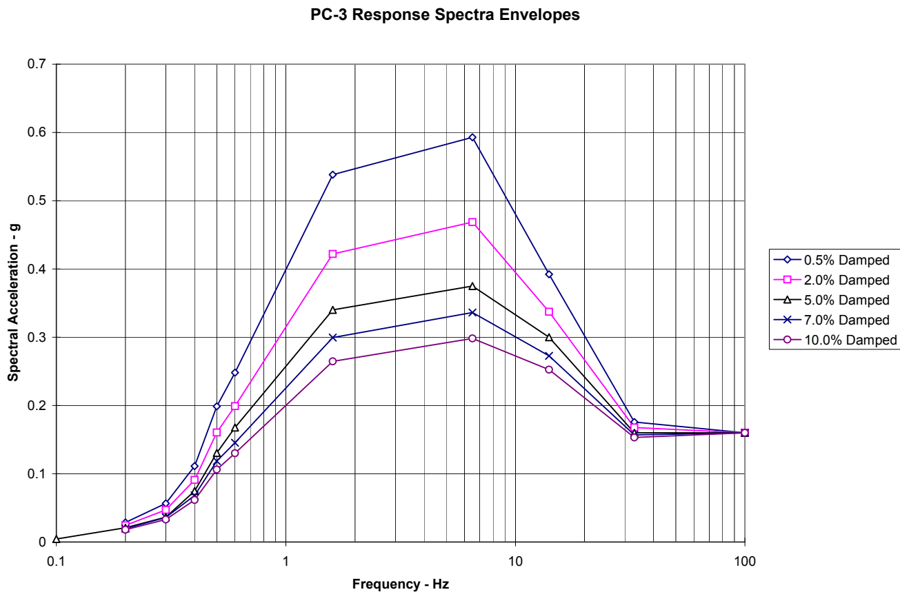
Figure 1.3.6-13. PC-3 Response Spectra Envelopes
