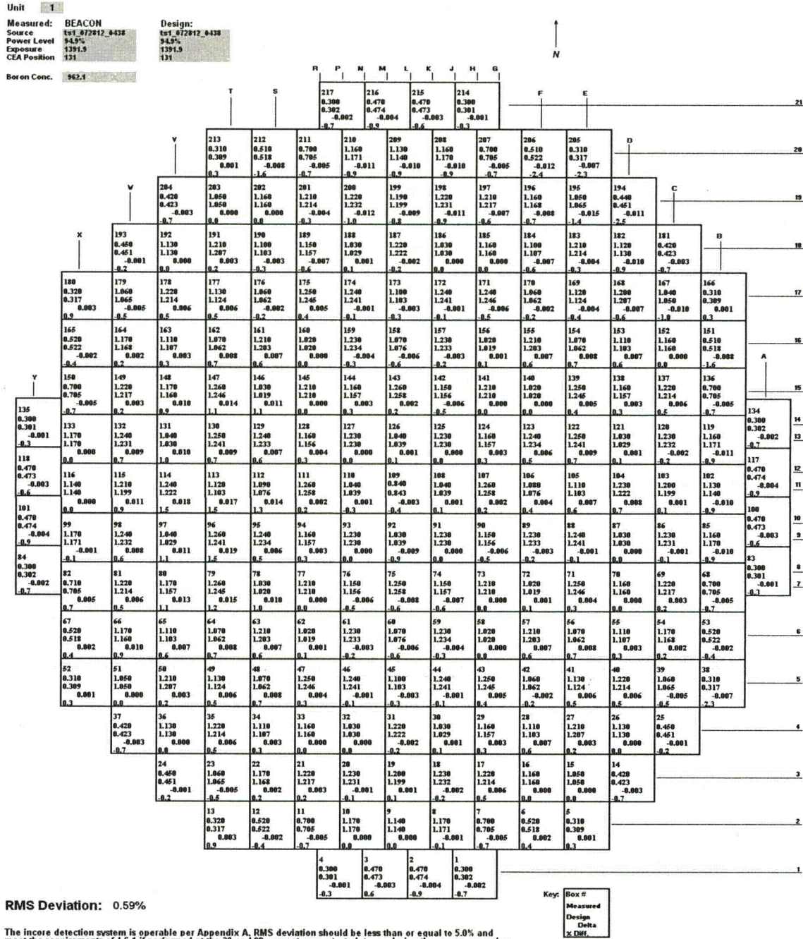
Figure 5 Cycle 24 - Power Distribution Comparison – 95% Power
