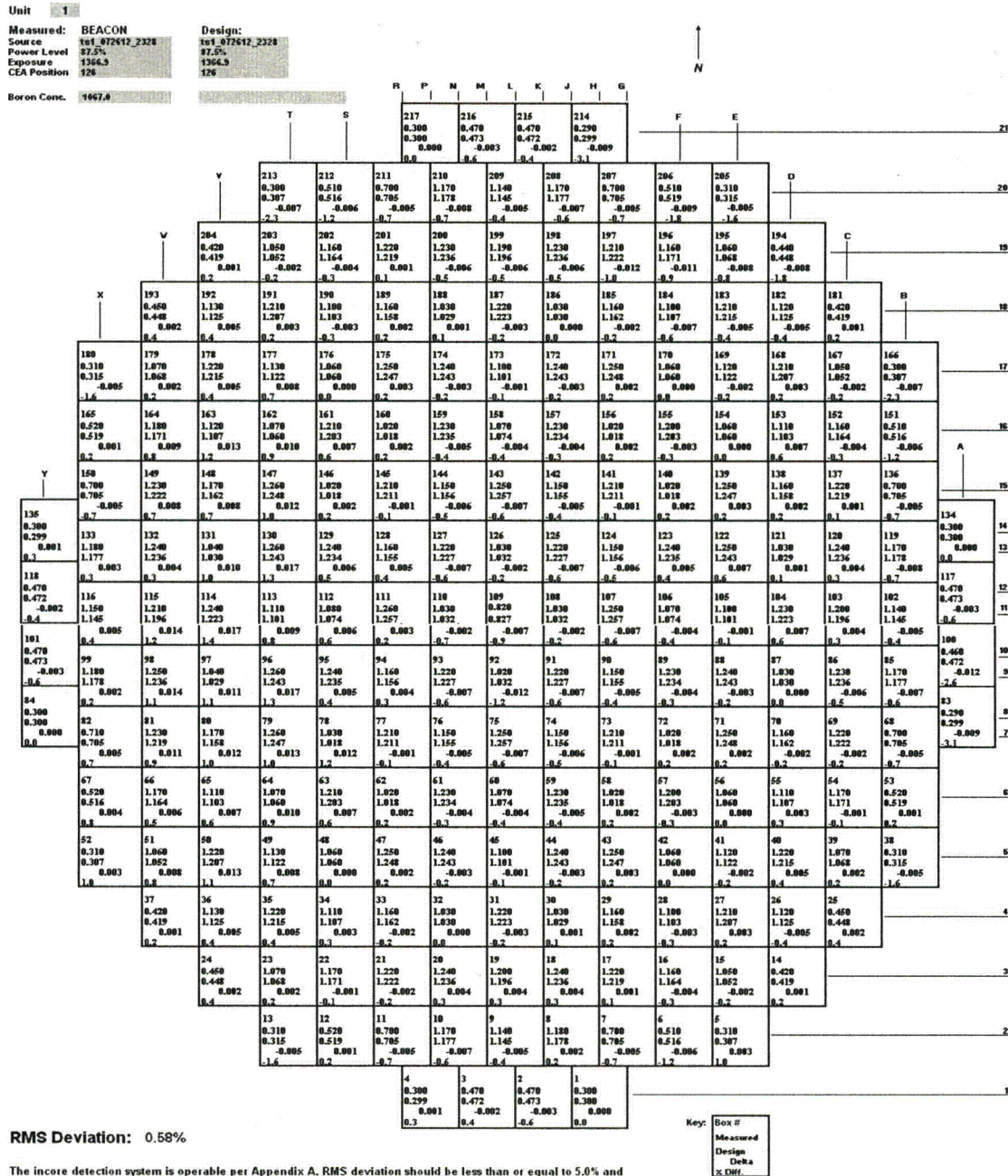
FIGURE 4 Cycle 24 - Power Distribution Comparison – 89% Power
