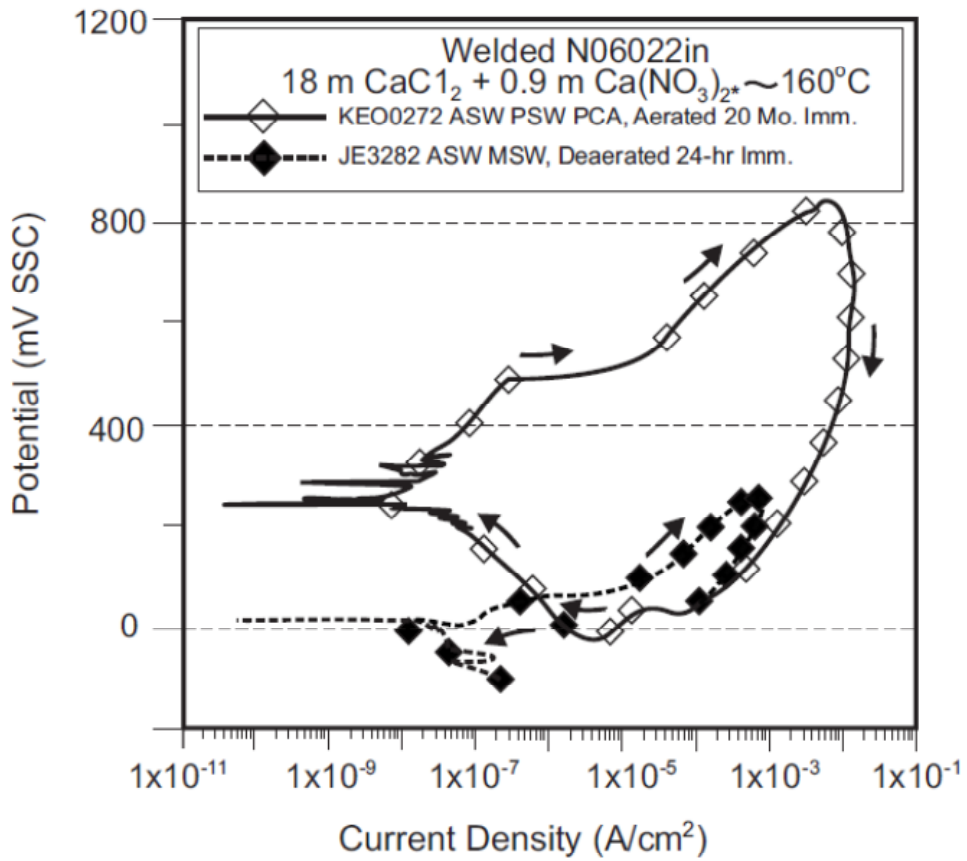
Figure 3. Cyclic Potentiodynamic Polarization for Alloy 22 in 18 M CaCl 2 + 0.9 mCa(NO 3 ) 2 , [NO 3- ]/[Cl - ] = 0.05 at ~ 160 °C [320 °F] Comparing Short and Long Term Immersion. Short Term Data Is At 160 °C [320 °F], Long Term at 155 °C [311 °F] [Rodriguez, et al., 18 permission by NACE]
