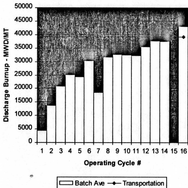
FUEL BURNUP VS CYCLE
