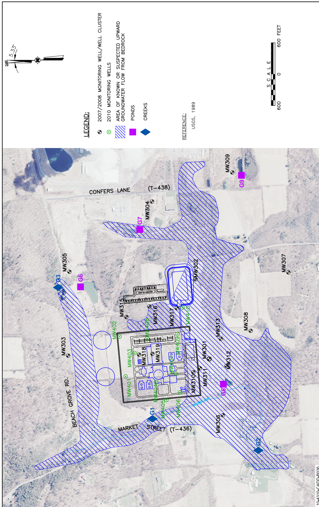
Figure 2.4-93 — {BBNPP Site Areas Known or Suspected of Having Upward-Flow of Groundwater from the Bedrock}
