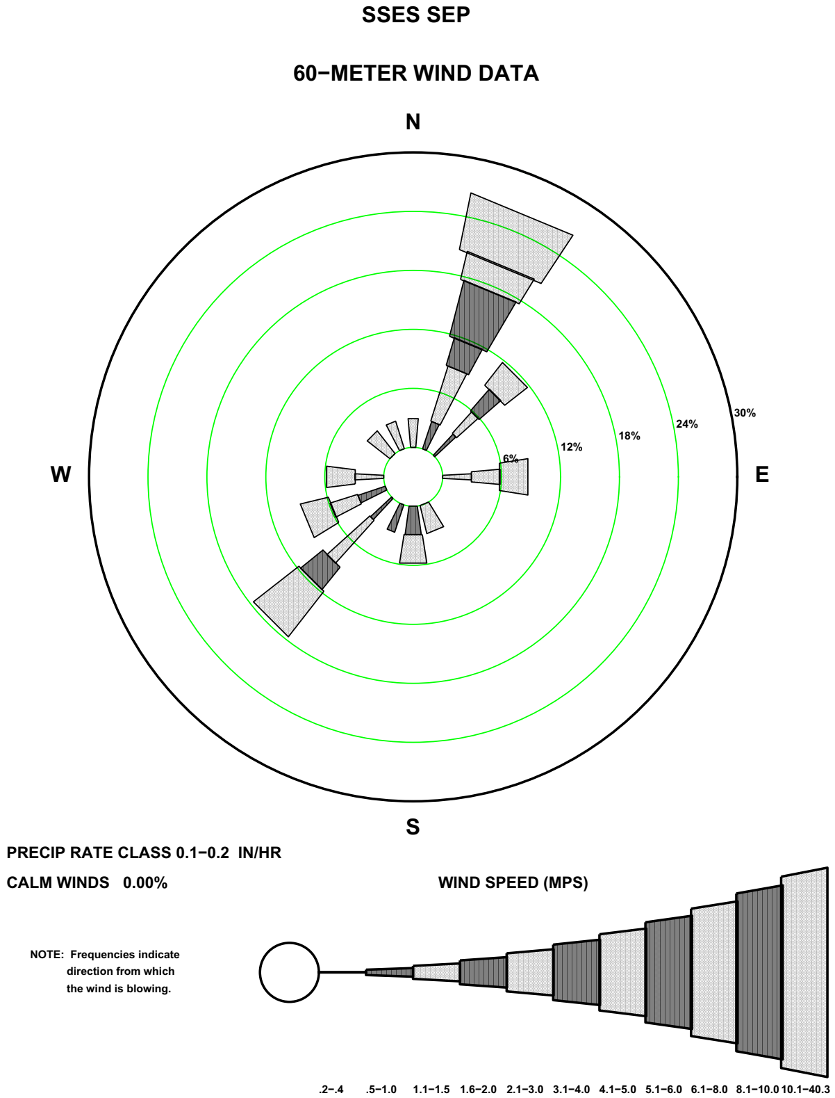
Figure 2.3-59— {BBNPP 197' (60-m) September Precipitation Wind Rose for Rate Class 0.1-0.2 in/hr}
