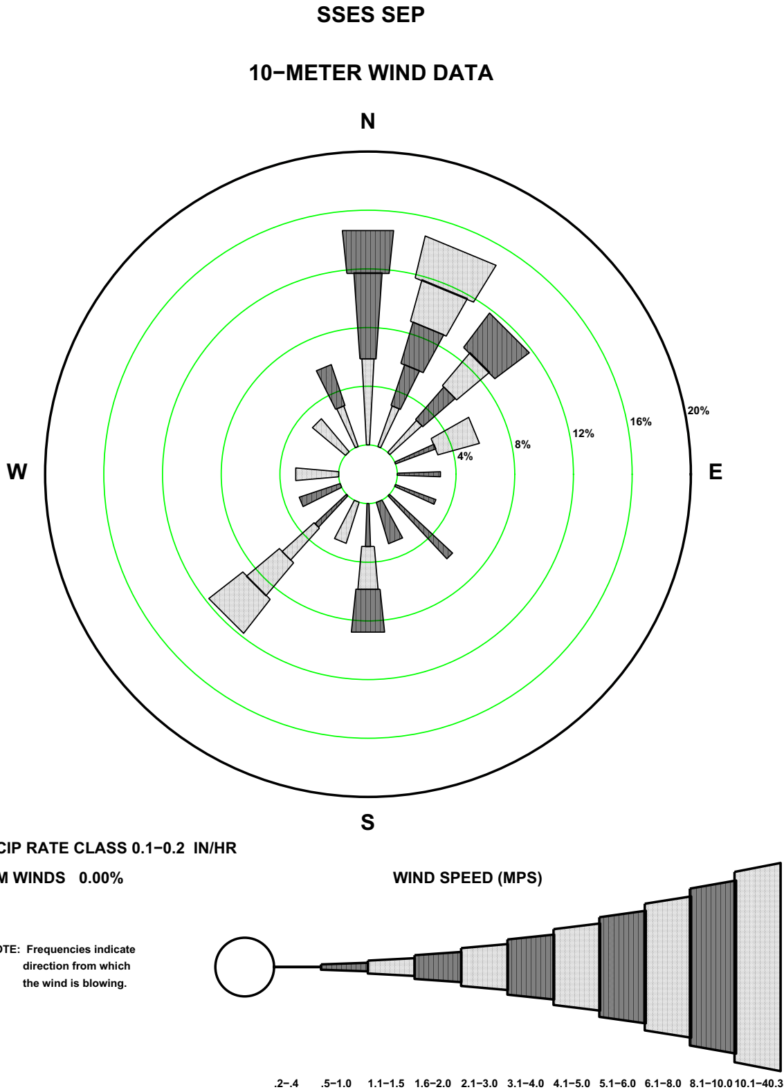
Figure 2.3-47— {BBNPP 33' (10-m) September Precipitation Wind Rose for Rate Class 0.1-0.2 in/hr}
