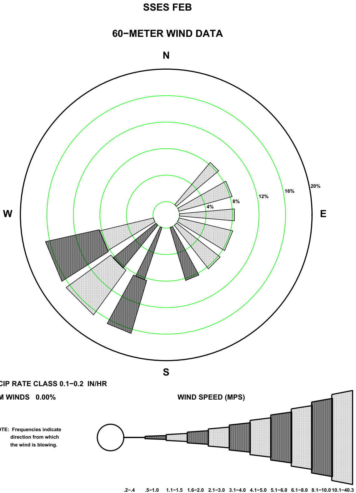
Figure 2.3-52— {BBNPP 197' (60-m) February Precipitation Wind Rose for Rate Class 0.1-0.2 in/hr}
