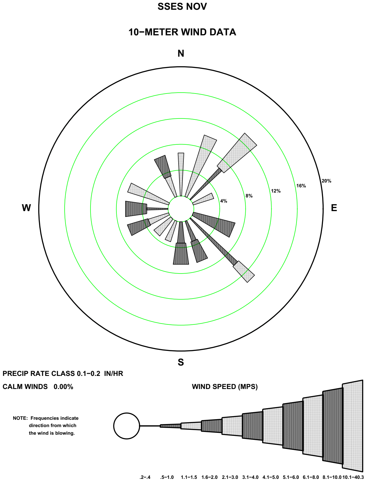
Figure 2.3-61— {BBNPP 197' (60-m) November Precipitation Wind Rose for Rate Class 0.1-0.2 in/hr}
