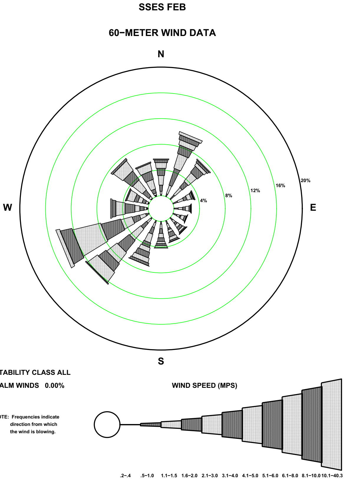
Figure 2.3-23— {BBNPP 197' (60-m) February Wind Rose}
