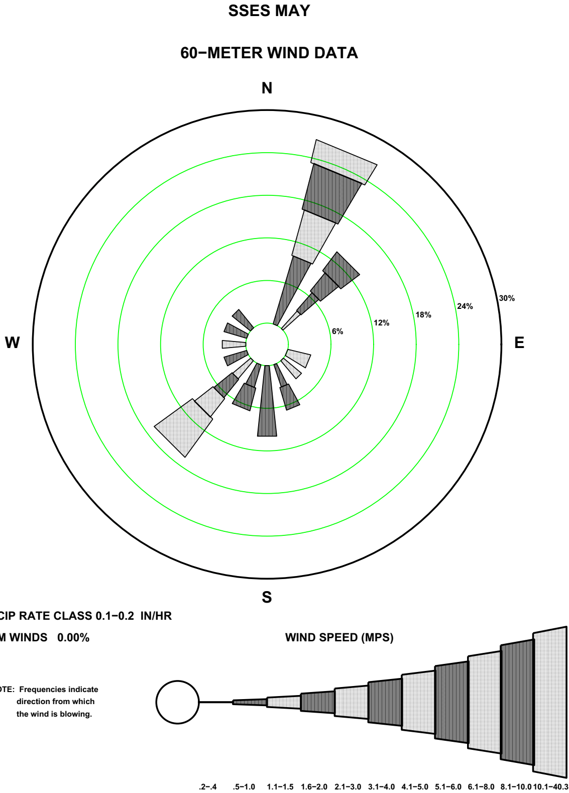
Figure 2.3-55— {BBNPP 197' (60-m) May Precipitation Wind Rose for Rate Class 0.1-0.2 in/hr}
