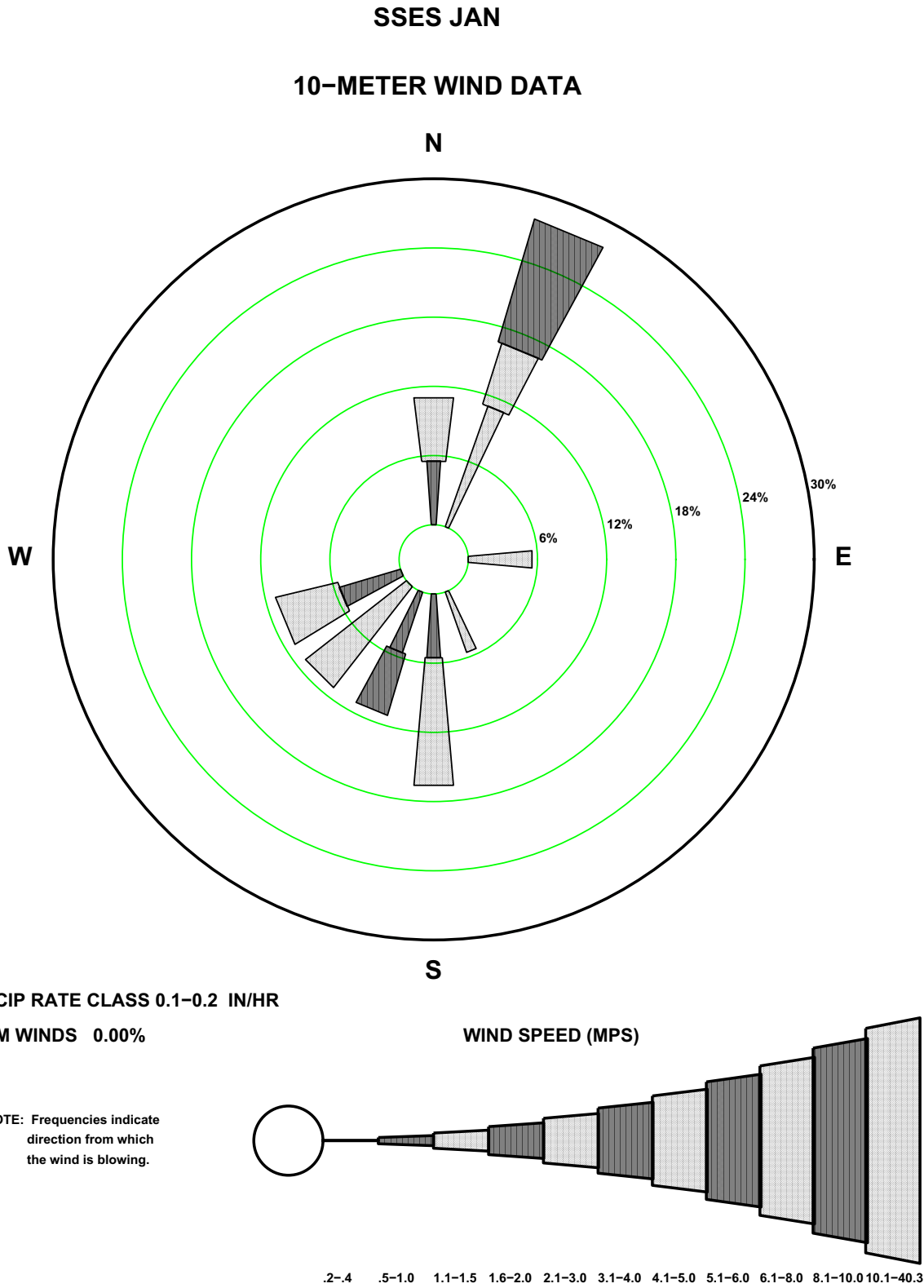
Figure 2.3-39— {BBNPP 33' (10-m) January Precipitation Wind Rose for Rate Class 0.1-0.2 in/hr}
